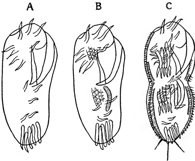
Figure 15. Reproduction and development in the infusorian Stylonychia , after Wallengren, 1901. A. Parent before division, showing the number and distribution of the locomotor appendages. B. Beginning of division: appearance of two groups of small projections, that are later to form by enlargement and distribution the appendages of the two offspring. C. Later stage of division: the two groups of embryonic appendages are scattering to take their final positions. The old appendages have not yet disappeared.
