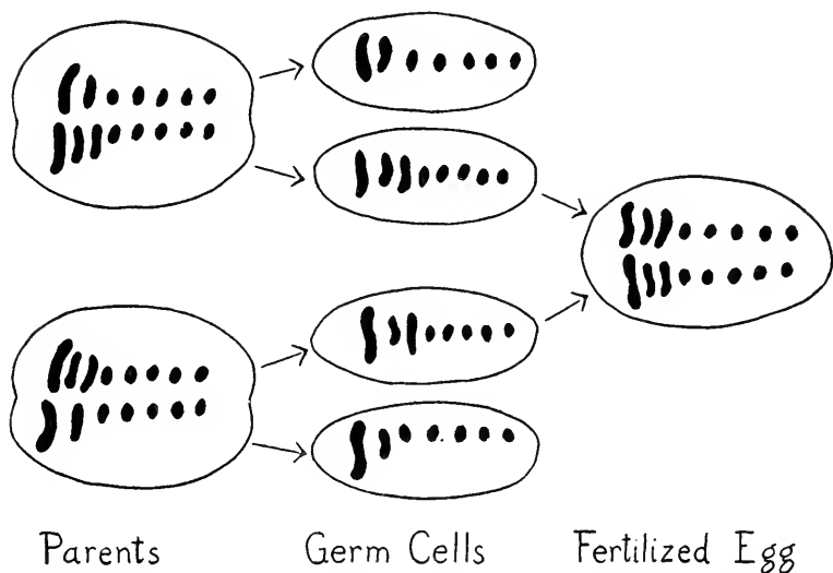
Figure 6. Diagram of the method by which there are produced individuals with four chromosomes in place of one of the pairs (in this case the second pair, counting from the left).
