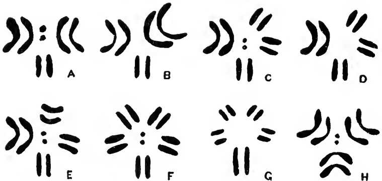
Figure 8. Diagrams showing the chromosome groups of eight different related species of flies, after Metz, 1916.
