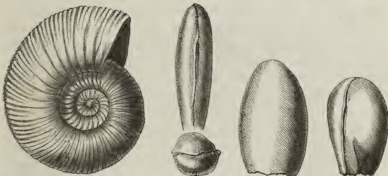
Fig. 58. Ammonites polyplocus . Reinecke. Fig. 59—61. Pholas Scheuchzeri (Bohrmuschel). Geinitz.
