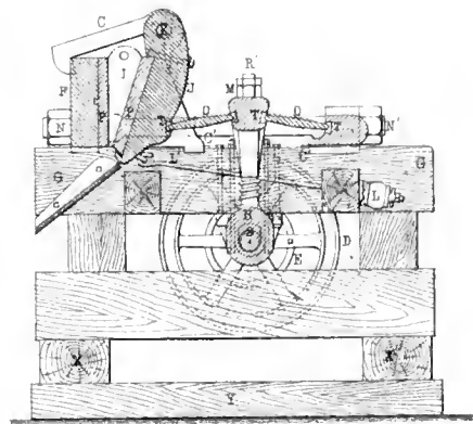
Fig. 4, VERTICAL SECTION
