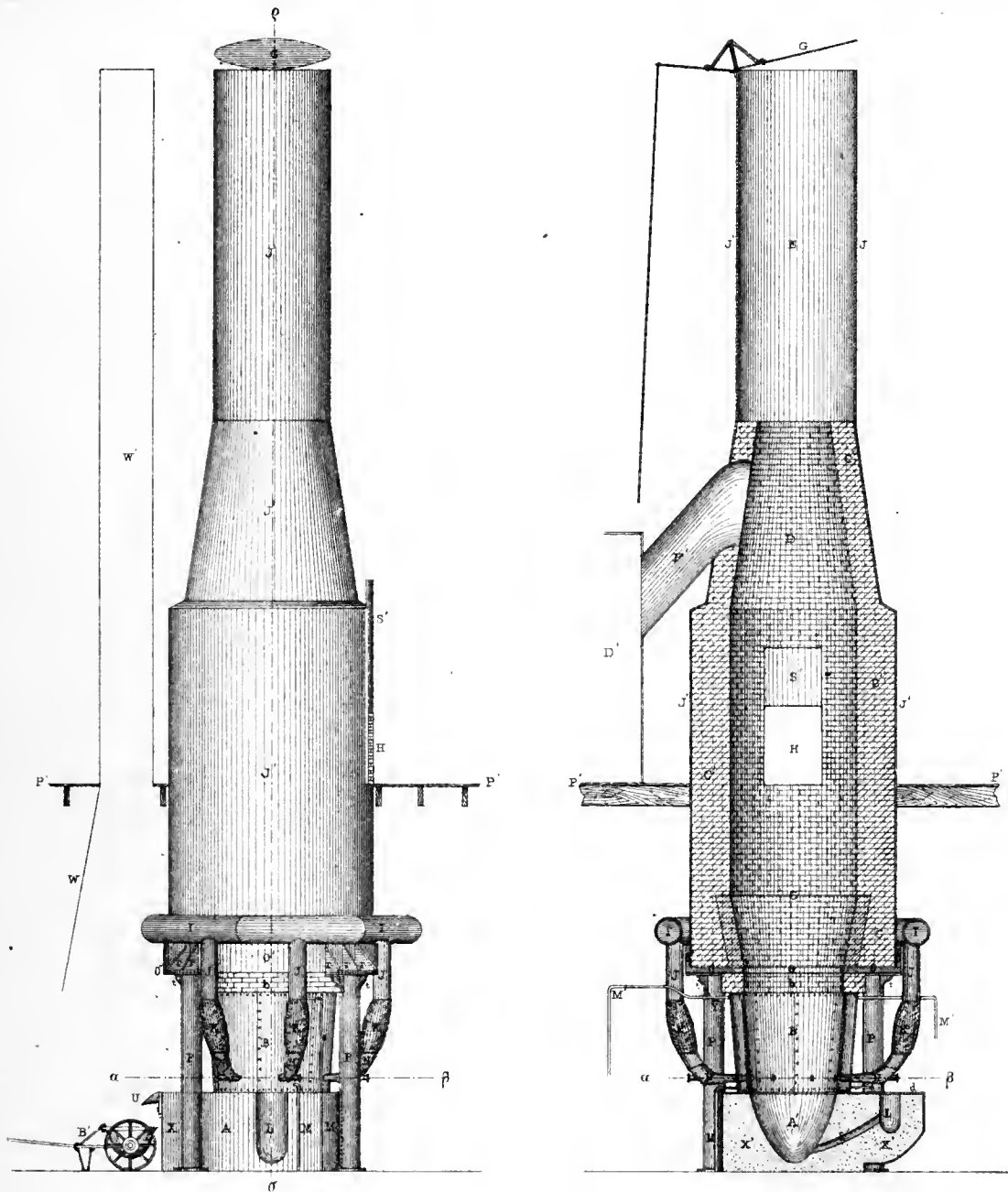
Fig 1 ELEVATION
