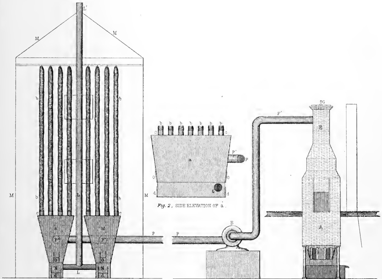
Fig. 1, ELEVATION.
