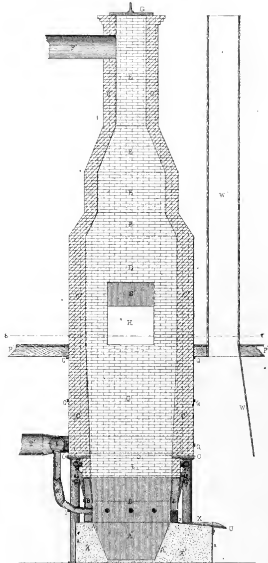
Fig. 3. SECTION ON Qσ
