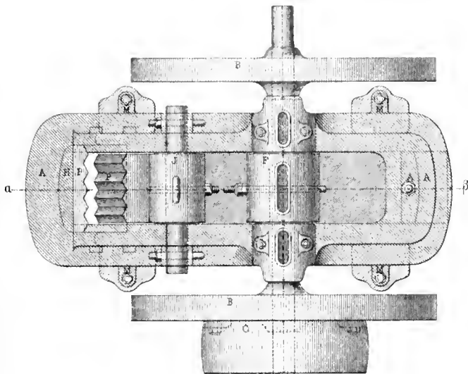
Fig. 1, HORIZONTAL PROJECTION
