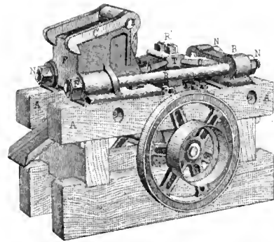
Fig. 3, PERSPECTIVE VIEW
