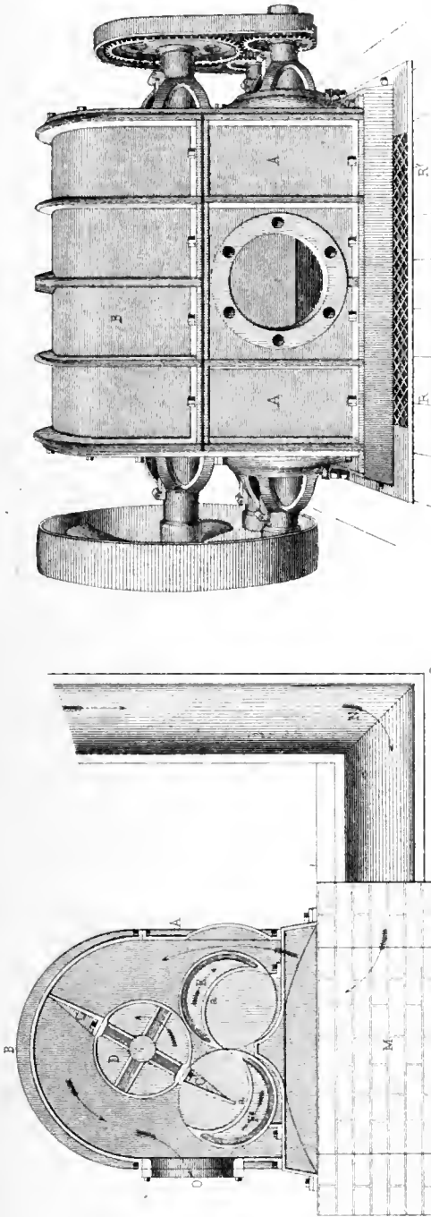
Fig. 1 PERSPECTIVE VIEW
