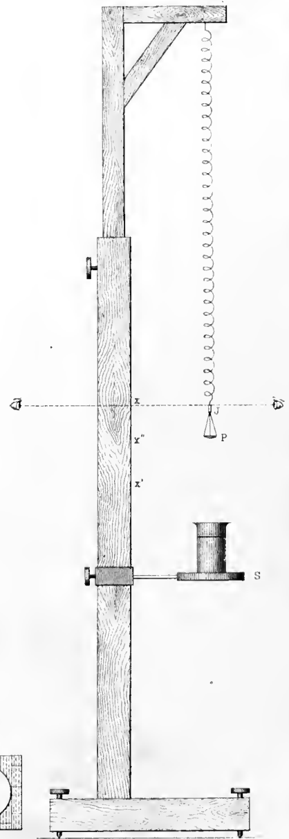
Fig. 2 JOLLY'S SPECIFIC GRAVITY SPRING BALANCE Scale: 1/8 ft - 1 in
