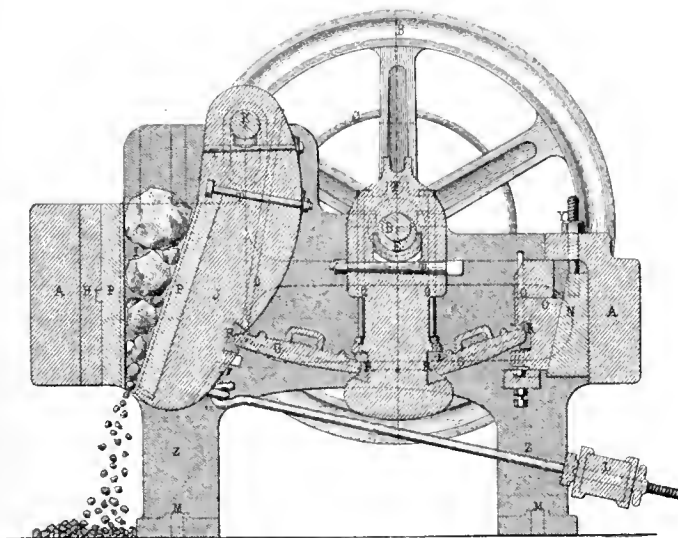
Fig. 2, SECTION ON αβ
