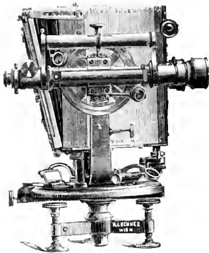
Abb. 50. Tachygraphometer.
