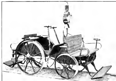
Abb. 304. Draisine, System Plank. [1825.]
