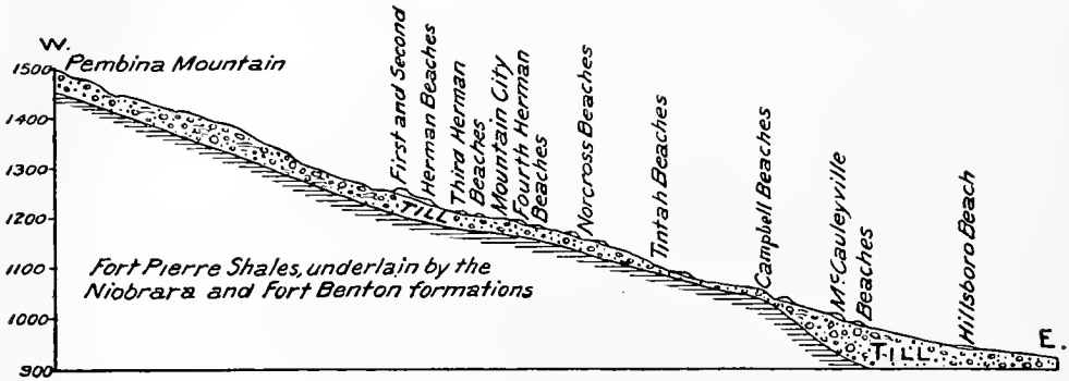
FIG. 29.—Section across ranges 6 and 5, Manitoba, 9 to 10 miles north of the international boundary. Horizontal scale, 2\frac{1}{2} miles to an inch.
