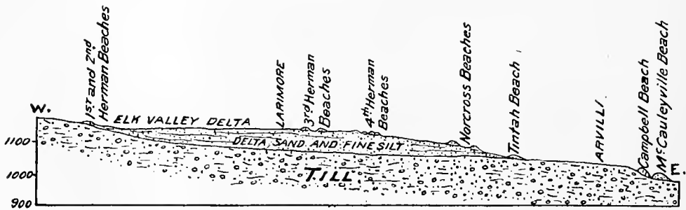
FIG. 25.—Profile across beaches in the vicinity of Arvilla and Larimore, N. Dak. Horizontal scale, 2½ miles to an inch.
