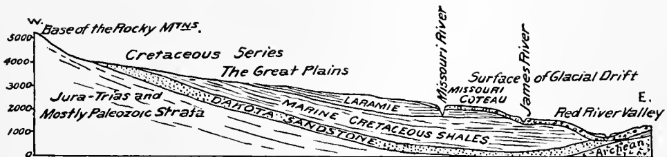
FIG. 33.—Section from the Rocky Mountains to the Red River Valley, showing the water supply of its saline artesian wells. Horizontal scale, 150 miles to an inch.
