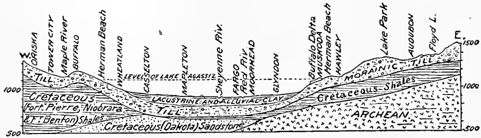
FIG. 3.—Section across the Red River Valley on the latitude of Moorhead and Fargo. Horizontal scale, 20 miles to an inch; vertical scale, 1,000 feet to an inch.
