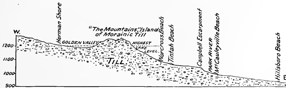
FIG. 27.—Profile across beaches at Park River, N. Dak., and westward. Horizontal scale, 2\frac{1}{2} miles to an inch.
