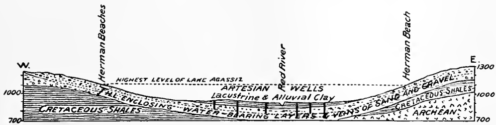
FIG. 32.—Section across the Red River Valley, showing the water supply of its fresh artesian wells. Horizontal scale, 15 miles to an inch.
