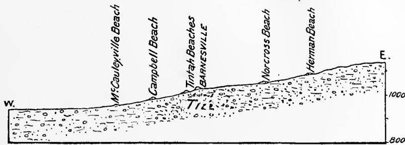
FIG. 20.—Profile across beaches at and near Barnesville, Minn. Horizontal scale, 2\frac{1}{2} miles to an inch.
