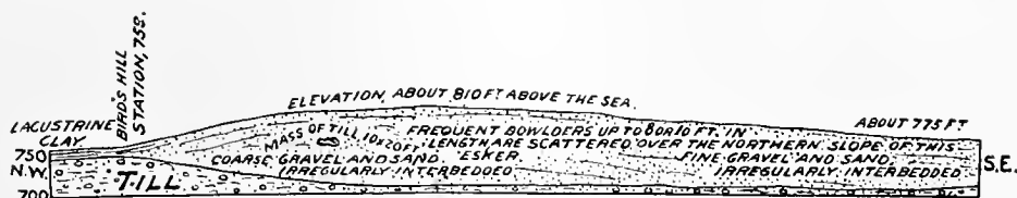
FIG. 10.—Section of Birds Hill. Horizontal scale, one-fourth mile to an inch.
