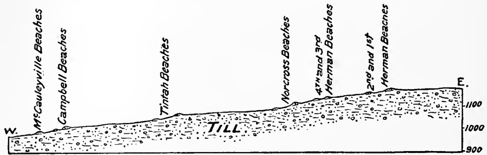
FIG. 22.—Profile across beaches on the north line of Onstead and Godfrey, Minn., west of Maple Lake. Horizontal scale, 2\frac{1}{4} miles to an inch.
