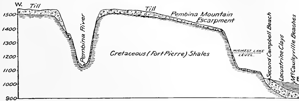
FIG. 28.—Section on the international boundary, south of ranges 6 and 5, Manitoba. Horizontal scale, 2\frac{1}{2} miles to an inch.
