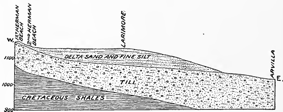
FIG. 14.—Section across the delta of the Elk Valley. Horizontal scale, 3 miles to an inch.
