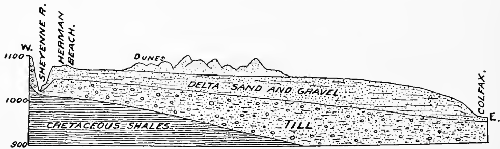
FIG. 13.—Section across the delta of the Sheyenne River. Horizontal scale, 6 miles to an inch.
