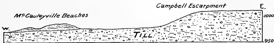
FIG. 21.—Section of the Campbell and McCauleyville beaches in sections 33 and 34, Liberty, Minn. Horizontal scale one-fourth mile to an inch.
