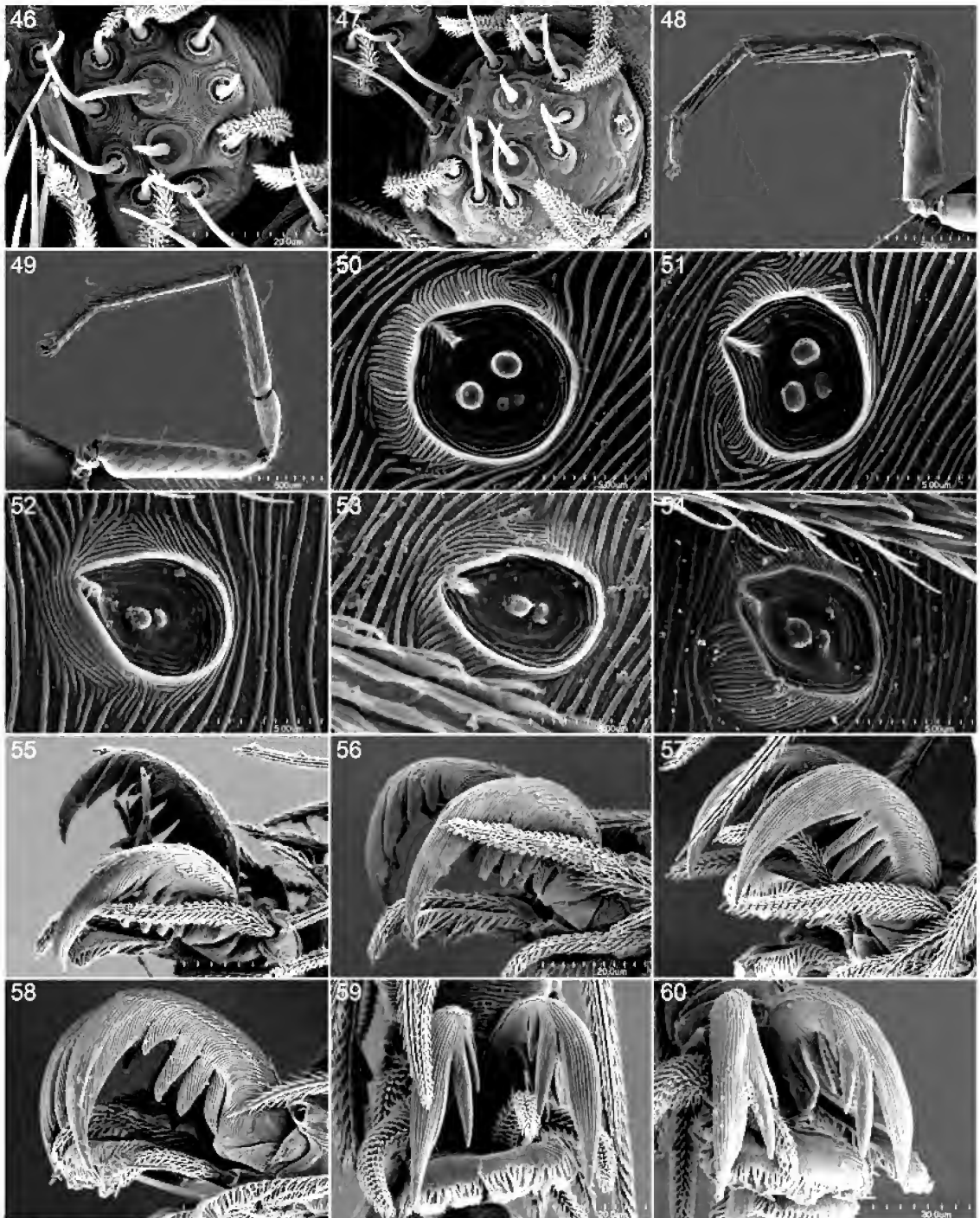
FIGURES 46–60. Simonoonops cranaea (Chickering), female. 46. Posterior median spinneret, apical view. 47. Posterior lateral spinneret, apical view. 48. Leg I, lateral view. 49. Same, leg IV. 50. Tarsal organ, leg I, dorsal view. 51. Same, leg II. 52. Same, leg III. 53. Same, leg IV. 54. Same, palp. 55. Claws of leg I, oblique lateral view. 56. Same, leg II. 57. Same, leg III. 58. Same, leg IV. 59. Claws of leg III, apical view. 60. Same, leg IV.
