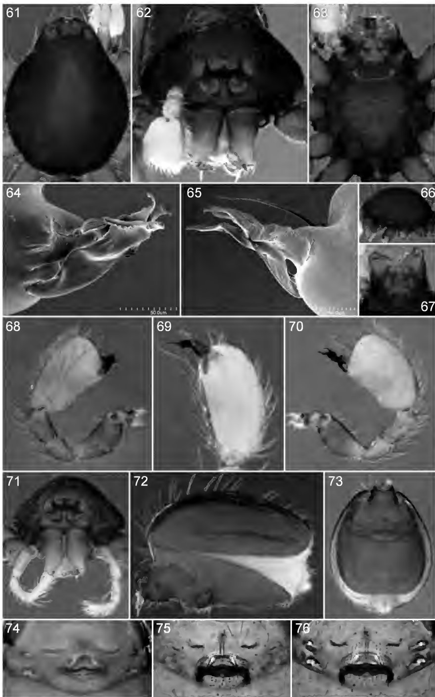
FIGURES 61–76. Simonoonops cranae (Chickering), male (61–70) and female (71–76). 61. Carapace, dorsal view. 62, 71. Same, anterior view. 63. Sternum, ventral view. 64. Left embolus, prolateral view. 65. Same, retrolateral view. 66. Carapace, lateral view. 67. Mouthparts, ventral view. 68. Left palp, prolateral view. 69. Same, ventral view. 70. Same, retrolateral view. 72. Abdomen, lateral view. 73. Same, ventral view. 74, 75. Genitalia, ventral view. 76. Same, dorsal view.
