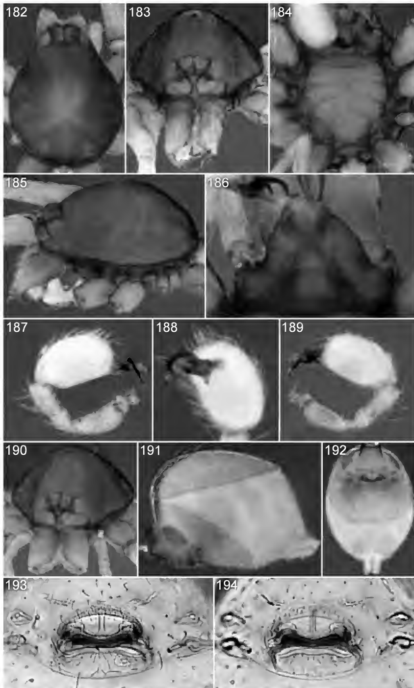
FIGURES 182–194. Simonoonops spiniger (Simon), new species, male (182–189) and female (190–194). 182. Carapace, dorsal view. 183, 190. Same, anterior view. 184. Sternum, ventral view. 185. Carapace, lateral view. 186. Mouthparts, ventral view, with oblique distal view of embolus. 187. Left palp, prolateral view. 188. Same, ventral view. 189. Same, retrolateral view. 191. Abdomen, lateral view. 192. Same, ventral view. 193. Genitalia, ventral view. 194. Same, dorsal view.
