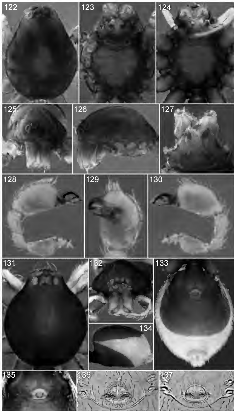
FIGURES 122–137. Simoonops lutzi , new species, male (122, 123, 125–130) and S. princeps (Simon), female (124, 131–137). 122, 131. Carapace, dorsal view. 123, 124. Sternum, ventral view. 125, 132. Carapace, anterior view. 126. Same, lateral view. 127. Mouthparts, ventral view. 128. Left palp, prolateral view. 129. Same, ventral view. 130. Same, retrolateral view. 133. Abdomen, ventral view. 134. Same, lateral view. 135, 136. Genitalia, ventral view. 137. Same, dorsal view.
