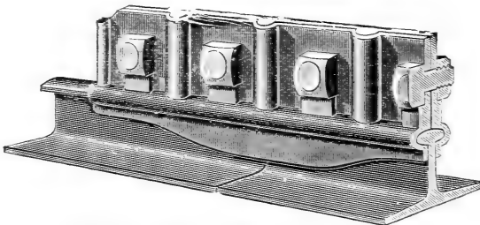
CROSS SECTION OF SPLICE.
