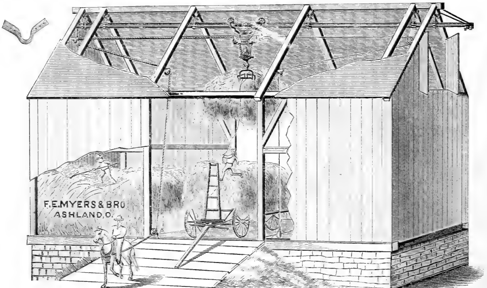
STEEL TRACK HAY CAR IN USE.
