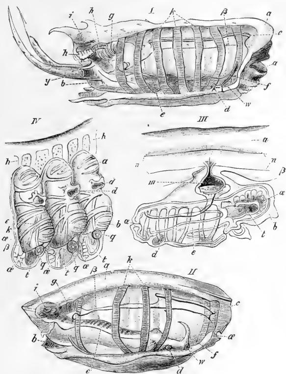
Fig. 172. — Salpa democratica-mucronata .
