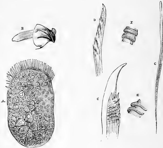
Fig. 55. — Polynoë squamata .
