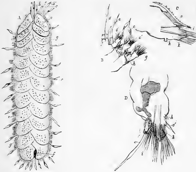
Fig. 54. — Polynoë squamata .
