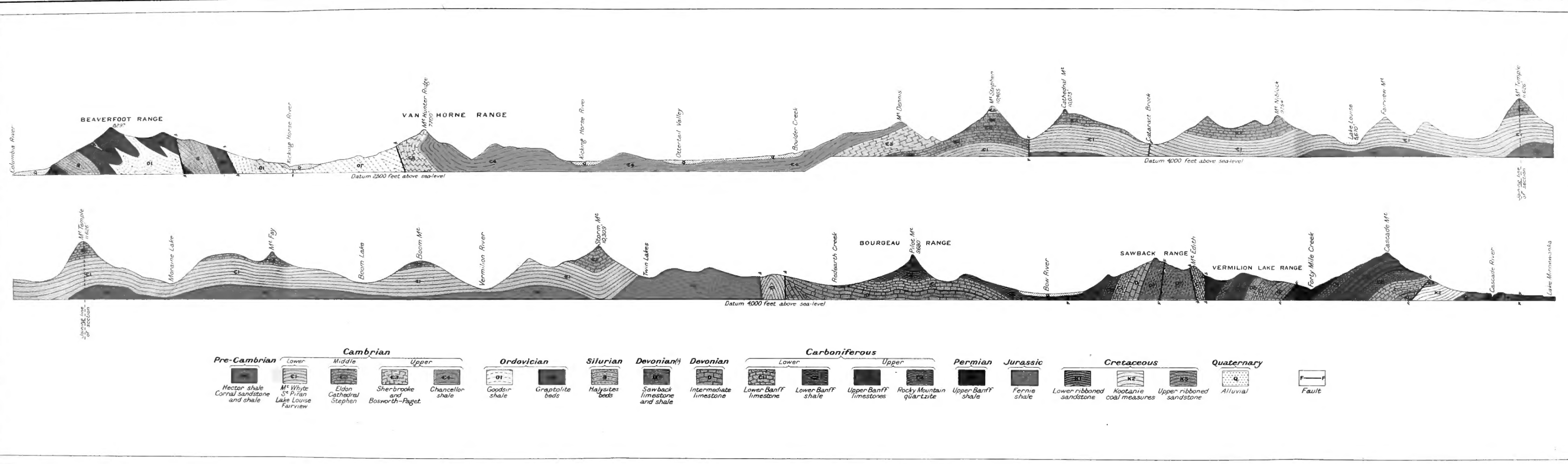
Structure Section across the Rocky Mountains near the Main Line of the Canadian Pacific Railway between the Cascade Trough and the Columbia Valley
