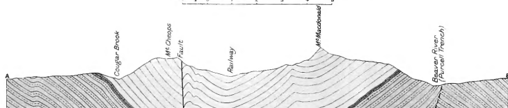
Section along line AB
