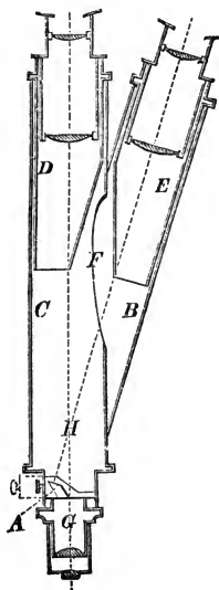
Fig. 6. Section of Binocular Microscope
