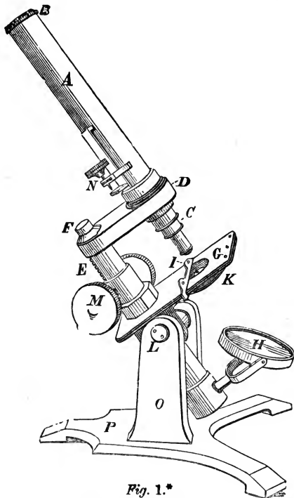
Compound Microscope.
