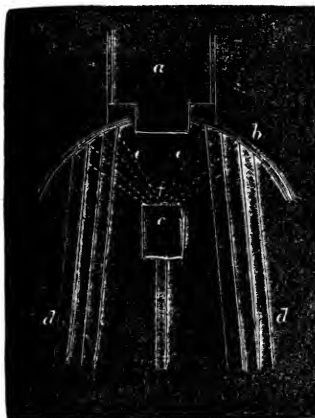
Fig. 11B Diagram illustrating the action of a " Lieberkühn ." a , object-glass; b , a concave silver reflector; c , a black spot ("dark well"); d, d , rays of light; e, e , the same reflected and brought to a focus at f .
