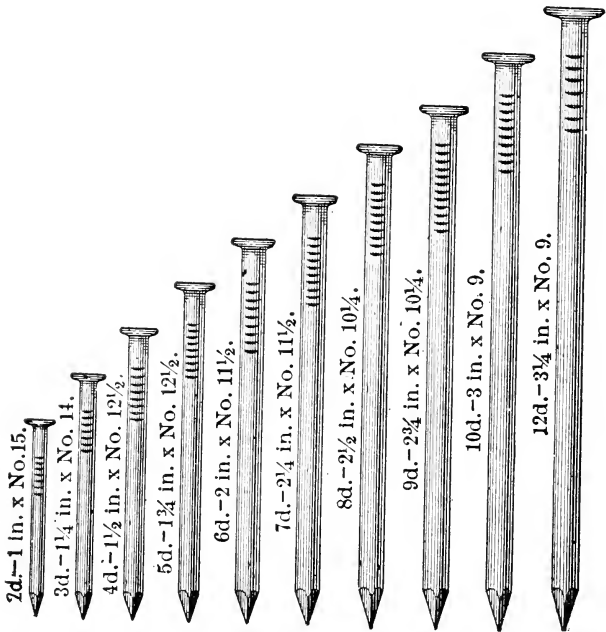
FIG. 235.—Wire nails.
