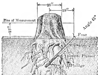
FIG. 66.—Correct location of charge in tap root.
