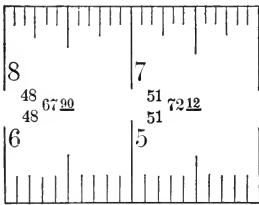
FIG. 115.—Rafter table.
