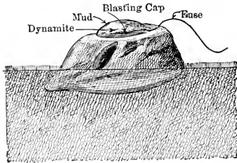
FIG. 63.—Mudcapping.
