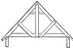
FIG. 82.—Self-supporting roof.
