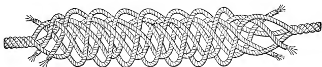
FIG. 229.—Permanent eye splice.
