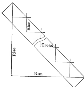
FIG. 120.—Stair string.
