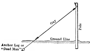
FIG. 30.—Guy for telephone pole.
