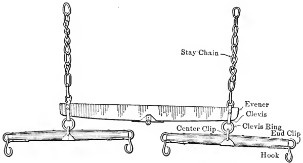
FIG. 152.—Evener and single trees.
