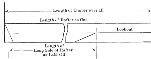
FIG. 119.—To cut rafter lookouts.
