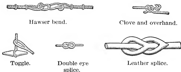
FIG. 230.—Splices.
