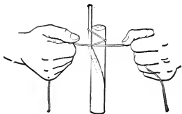
FIG. 62.—Tying the fuse into the cartridge.
