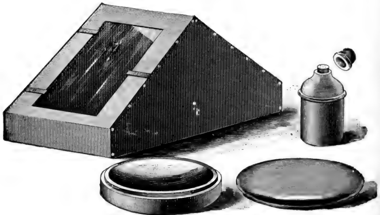
Artificial Horizon.*
