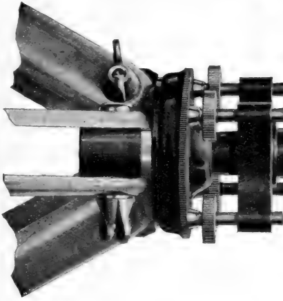
Engineers' 18-inch Wye Level. (Power 35 diameters.) As made by C. L. Berger & Sons.
