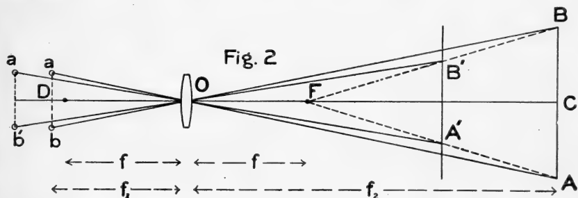
Figure 2 shows a section of a telescope provided with stadia wires.
