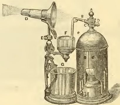
Steam atomizer.
