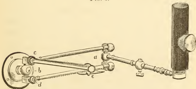
Mackenzie's bracket-light, with concentrator.
