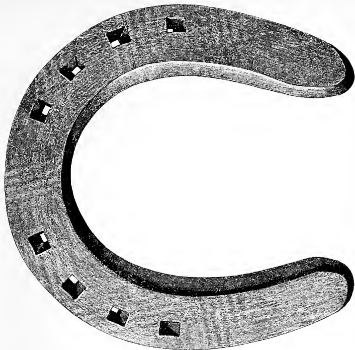
FIG. 247.—Cart horse stamped fore shoe (for show purposes). Made from 1\frac{1}{2} \times \frac{3}{4} inch iron.
