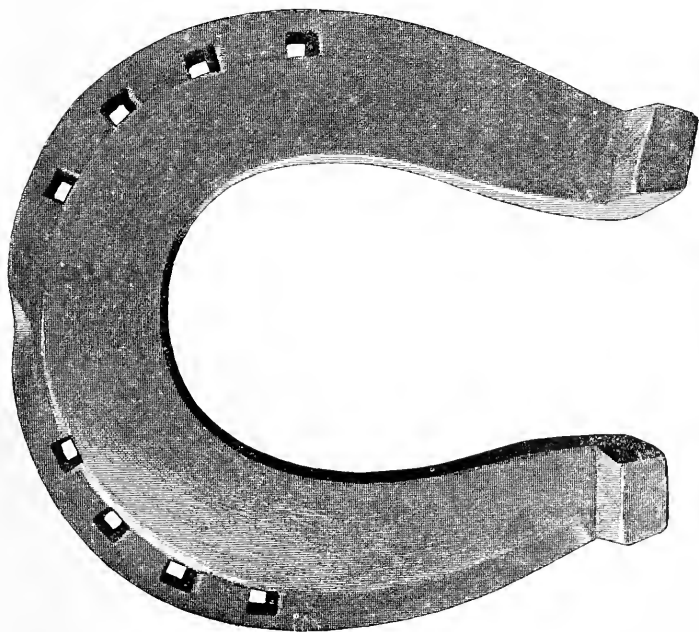
FIG. 325.—Stamped fore shoe (for cart horse), 'set' around outer margin. Made from 1\frac{1}{2} × \frac{5}{8} inch iron.
