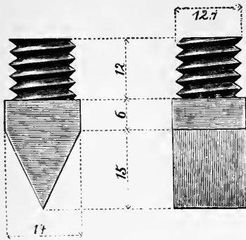
FIG. 115.—Screws (full size) provided with Whitworth thread.
