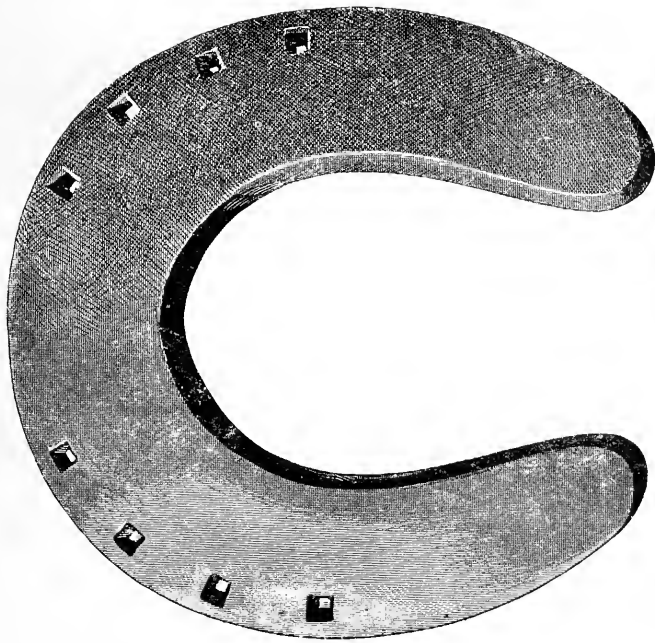
FIG. 324.—Stamped fore shoe (for cart horse). The 'quoit' shoe. Made from 1\frac{1}{2} × \frac{5}{8} inch iron.
