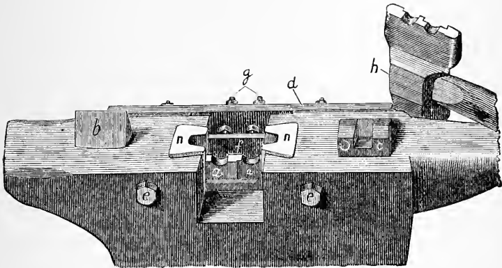
FIG. 114.—Anvil for making screws. a , mould for forming shank; b , cutter; c , mould for making sharp-headed screws; d , plate carrying set screws, g , and held in position by the two screws, e , e ; f , die carrying the moulds, a , a . This can be set at any distance from the plate, d , by moving the set screws, g . The length of the shank is thus fixed; h , forging hammer.
