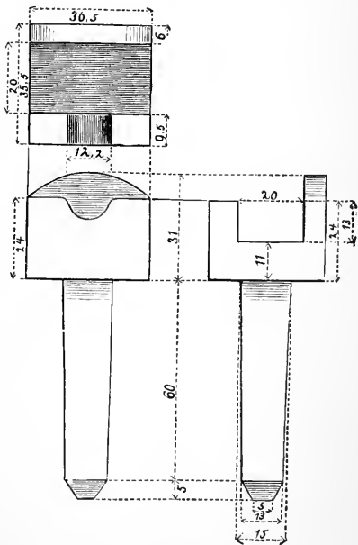
FIG. 119.—Mould for making screws. Army pattern for field use.
