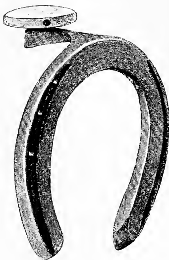
FIG. 234.—Partially fullered fore shoe (for trotters). Made from \frac{3}{4} \times \frac{1}{2} inch iron.
