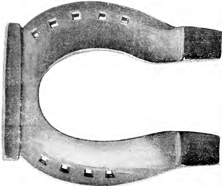
FIG. 250.—'North Country' stamped hind shoe. Made from 1\frac{1}{2} \times \frac{1}{2} inch iron.
