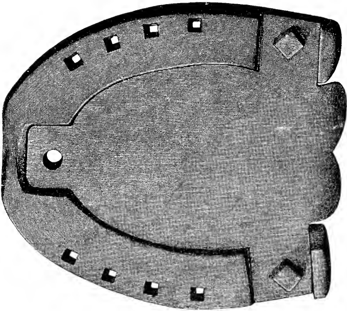
FIG. 360.—Stamped cart hind shoe (surgical), with arrangement for dressing foot. Made from 1\frac{1}{4} \times \frac{1}{2} inch iron.
