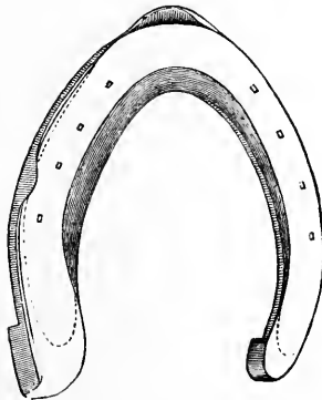
FIG. 266.—Left hind shoe for horse with turned-in toes. The outer branch is seen to be wider than the inner. The dotted lines indicate the bearing of the hoof.
