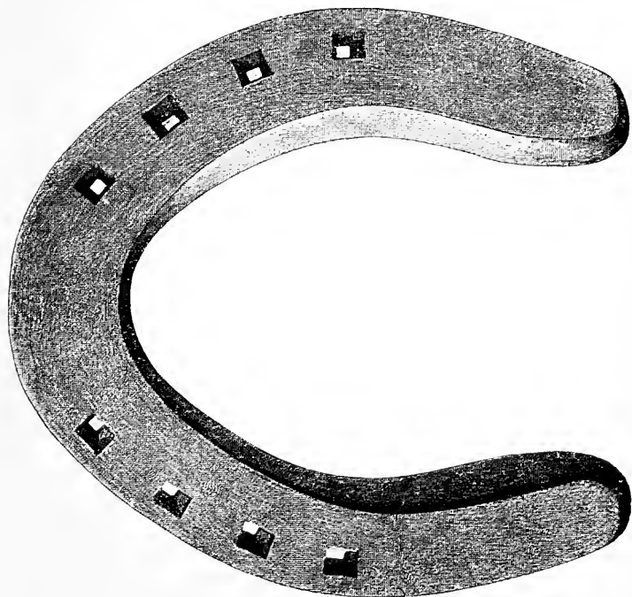
FIG. 248.—Cart horse stamped hind shoe (for show purposes). Made from 1\frac{1}{2} \times \frac{3}{4} inch iron.
