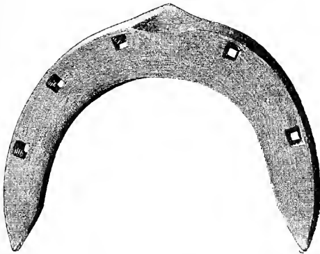
FIG. 260.—Stamped fore tip. Made from \frac{3}{4} \times \frac{3}{8} inch iron.
