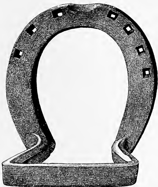
FIG. 393.—Stamped patten fore shoe. Made from \frac{3}{4} \times \frac{1}{2} inch iron.
