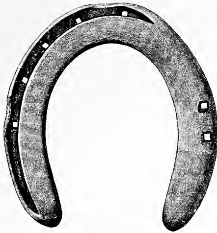
FIG. 292.—Fullered seated feather-edged fore shoe. For harness or riding. Made from \frac{7}{8} \times \frac{1}{2} inch iron.
