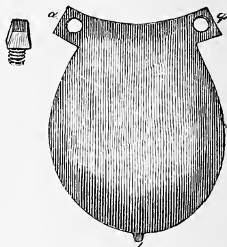
FIG. 356.—Cover for shoe shown in previous fig. The letters indicate similar points.
