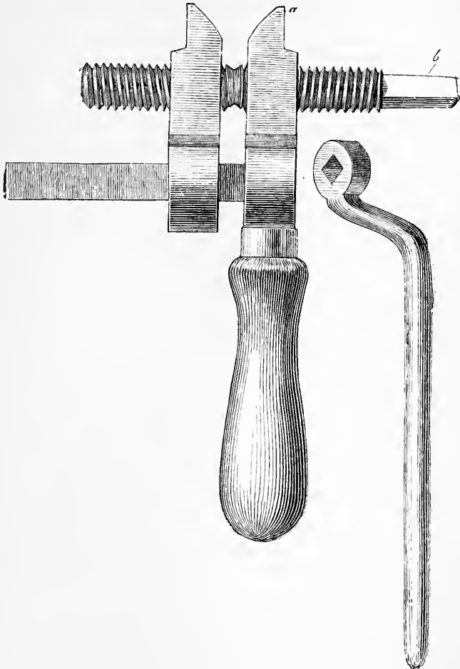
FIG. 334.—Instrument for expanding De Fay's shoe. a , the iron checks which fit between the heels of the shoe; b , square head on the right and left-handed screw, for taking the key.
