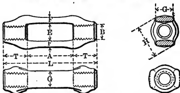
Dimensions of Bar.
