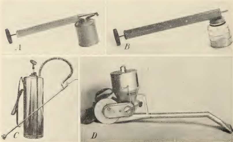
FIGURE 160.—Spraying and dusting equipment: A , Hand atomizer; B , hand duster (both useful for small gardens); C , compressed-air sprayer; D , rotary fan or blower type of duster (the last two useful for larger gardens).
