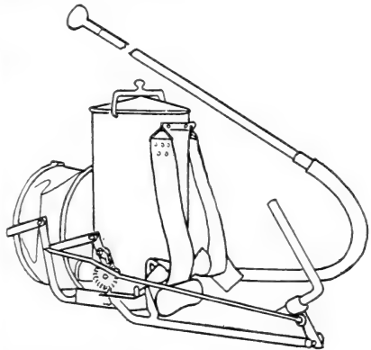
FIGURE 170.—Knapsack-bellows duster.
