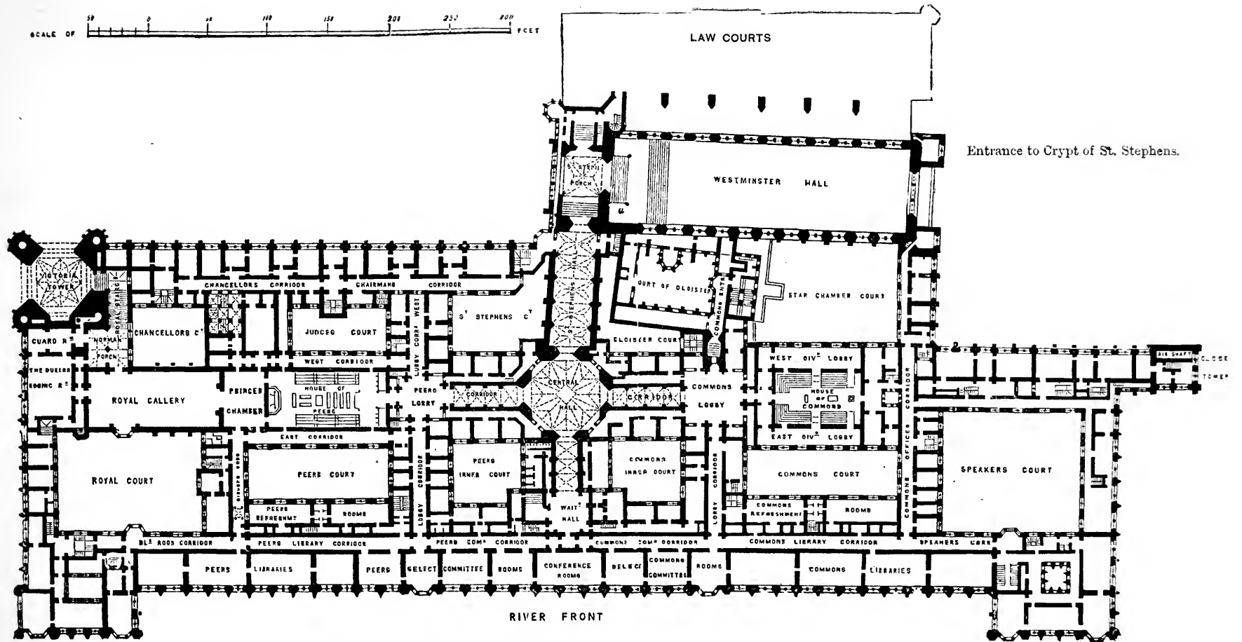
GROUND PLAN OF THE HOUSES OF PARLIAMENT. SIR CHARLES BARRY, R.A., ARCHITECT.
