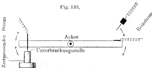
Helmholtz'sche Wippe.
