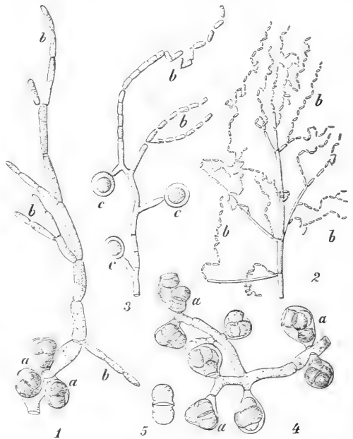
Fig. 50. Endomyces decipiens REESS.
