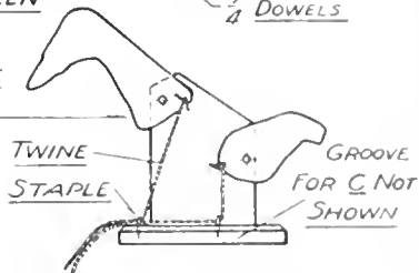
VIEW OF PARTS WITHOUT C IN PLACE
