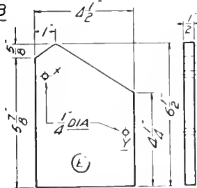
VIEW OF PARTS WITHOUT C IN PLACE
