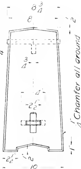
Detail of mortise and tenon at A.
