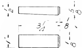
Detail of key
