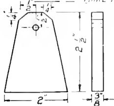
PART C MAKE TWO
