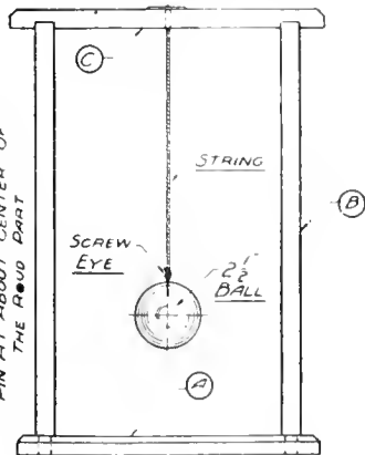
PARTS ASSEMBLED BUT WITHOUT PIN IN PLACE
