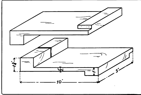
Fig. 179. Bench-Hook.
