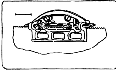
Fig. 97. A Saw-Jointer.
