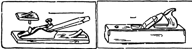
Fig. 99. Adjustable Chisel-Gage. Fig. 100. Wooden Bench-Plane.
