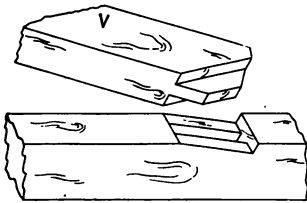
67 Oblique mortise-and-tenon
