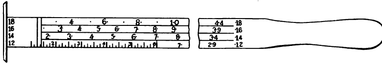
Fig. 199. Lumberman's Board Rule.
