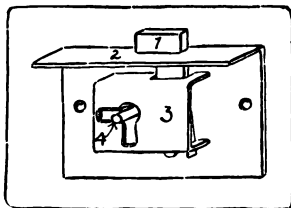
Fig. 236. Rim-lock, for Drawer. 1. Bolt. 2. Selvage. 3. Box. 4. Key-pin.
