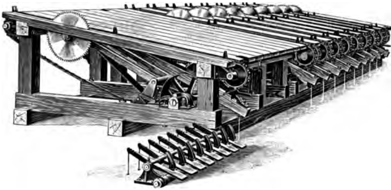
Fig. 45. Automatic Gang Lumber-Trimmer. It may be set to cut automatically to any desired length.
