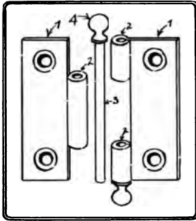
Fig. 234. Parts of a butt-hinge. 1.1. Leaves. 2.2. Knuckle. 3. Pintle. 4. Acorn.
