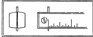
Fig. 212. Spur of Marking-Gage.
