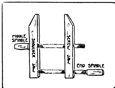
Fig. 173. Handscrew.
