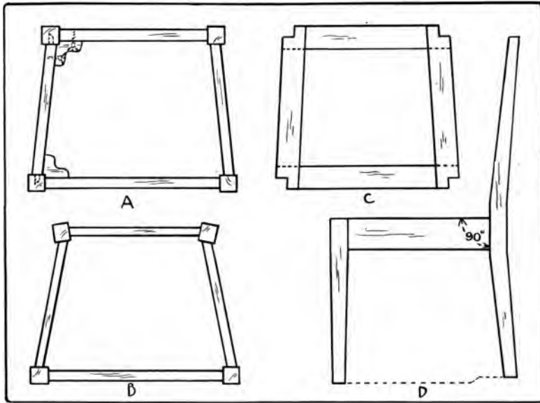
Fig. 298. Chair Construction.
