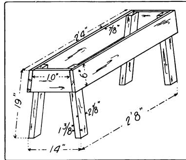
Fig. 171. Saw-Horse.
