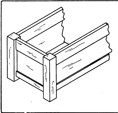
Fig. 290. Chest Construction.
