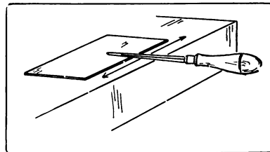
Fig. 157. Resharpening a Cabinet-Scraper: Flattening the Edge.
