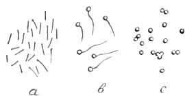
Fig. 3. Bacillus cellulosaemethanicus .
