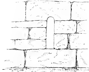
Fig. 146. Outside elevation of a slit window.
