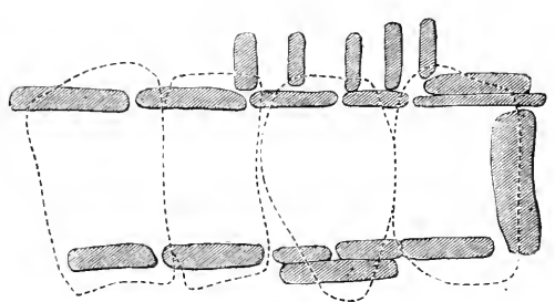
Figs. 85 and 86. Elevation and Plan of Calliagh Dirra's House.
