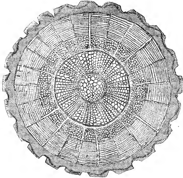
Fig. 76.— Sigillaria vascularis (Diagrammatic section). 1
