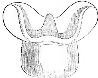
Fig. 93.— Succinea elegans .
