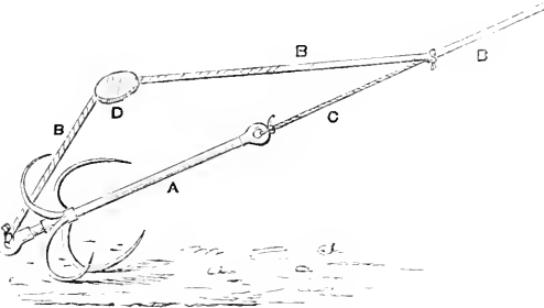
Fig. 35.—Position of grapple at work: A, grapple; B, main cord of ditto; C, safety-cord of ditto; D, cork to keep B from fouling the hook.
