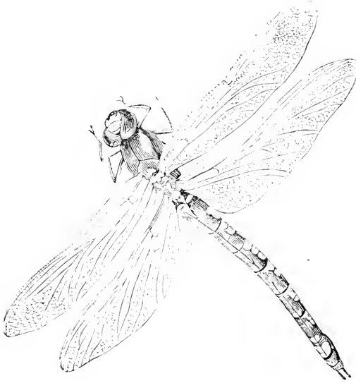
Fig. 27.—Dragon-fly.
