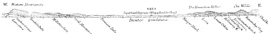
Fig. 99.—Diagram showing geology west to east across Yorkshire.
