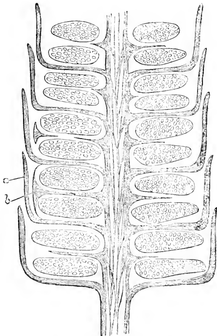
Fig. 135.—Vertical Section of Fruit of Calamite. ( c , protective bracts; b , peltate scales.)
