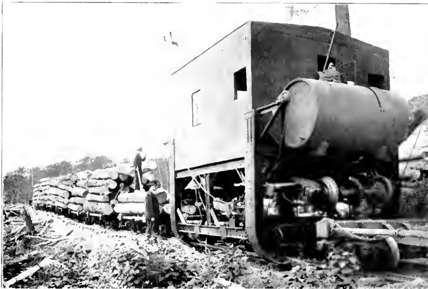
THE McGEFFERT STEAM LOG LOADER.
