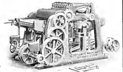
26" DOUBLE SURFACER
