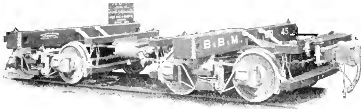
STANDARD LOGGING CAR, MANUFACTURED BY THE RUSSEL WHEEL & FOUNDRY COMPANY
