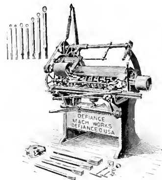
32 IN. AUTOMATIC SPOKE LATHE.
