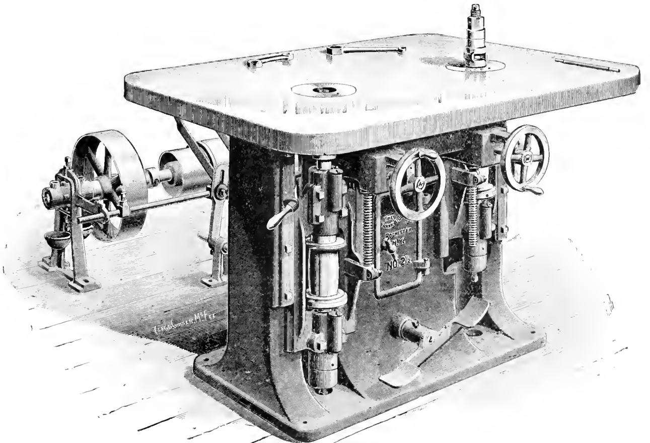
Fig. 929—Clement No. 2½ Two-Spindle Shaper.
