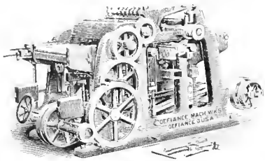
26" DOUBLE SURFACE PLANER. Planes 26" wide x 12" deep. Has Cut Gears throughout. Has Sectional Feed Roll and 12" Ring Oiling Bearings.
