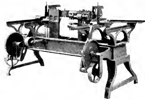
COMBINED END MATCHER BUILT BY A. J. SCHINDLER, CHICAGO.
