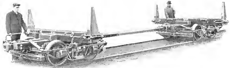
LOGGING CAR FTTED WITH RUSSEL TRIP STAKE HOLDERS
