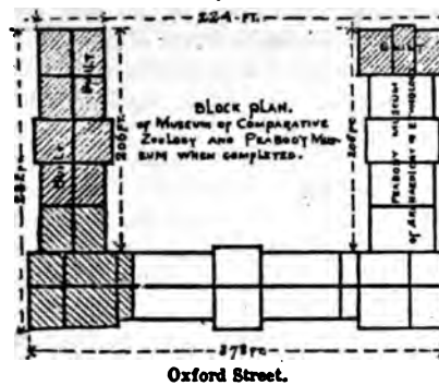
Ground Plan of Projected Museum (26).
