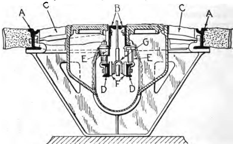
FIG. 3,693. —Yoke construction for conduit or underground trolley, as installed on Metropolitan Railways, New York City. These yokes were placed 5 feet apart in an excavation made through the street. The track rails A, A, and the slot rails B, B, were then laid on the yokes, and the ties C, C, inserted. The whole structure was then blocked up, surfaced and lined, and constituted the track construction. The conductors consist of two channel beams, D, D, placed 6 inches apart and supported by insulators E, E, at each yoke. The contact rail joints are bonded in a manner somewhat similar to ordinary rail bonding, and from a complete metallic circuit having a pressure of 500 volts between the conductors. The current from these conductors passes through the slot or opening between the slot rails and extends into the conduit to a distance sufficient to bring the plow contacts or shoes F, against the conductors. The spring G, tends to keep the shoes normally about 8 inches apart, so that when they are pressed into the 6 inch space between the conductors, they maintain a firm sliding contact with the latter. The yokes used on some of the lines constructed later are practically the same, but T iron conductors are used instead of the channel beams. In order to provide of expansion and contraction the center of each section of rail is fastened solidly to an insulator at that point, and the ends of each rail are slotted and bonded with a flexible bond. Hand hole provided with iron covers are placed about 15 feet apart directly over the insulators. The manholes are placed about 150 feet apart, and usually between the tracks. Arrangements are made at these points to drain the conduit into the sewers. The bottom of the conduit is given a minimum grade of 2 inches to 100 feet, so as to insure proper drainage on sections of level track. The contact rails are treated like a double trolley wire, and the feeders and mains are laid in underground conduits. This system is so expensive to install that its use is limited to only a few of the largest cities where for various reasons the use of the overhead trolley is objectionable and prohibited.
