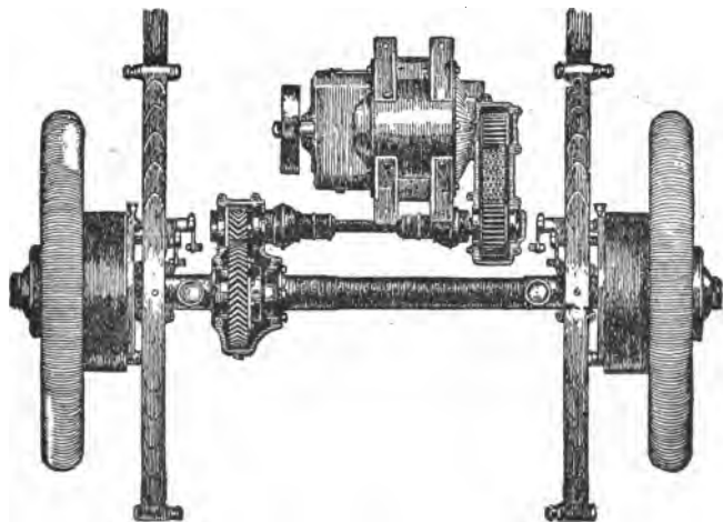
FIG. 4,070. —Waverly double reduction gear or combination herringbone gear and "silent" chain. In construction the motor shaft is parallel to the intermediate or jack shaft and drive shaft. Two universal joints are used, so as to give freedom of motion in any direction. The motor weight is above the springs. The first reduction is by the silent chain enclosed in a casing at end of motor; the second reduction is through the herringbone gear in the axle.
