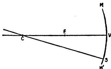
FIGS. 3,771 and 3,772.—Concave spherical mirror; definitions. In the diagram V is the vertex; MM', the aperture; CV, the principal axis; CS, a secondary axis; C, center of curvature; F, principal focus (midway between V and C). Any line drawn from C to the mirror will be perpendicular to the mirror at that point. This line then will always be the normal which will be used in making the angle of incidence equal to the angle of reflection. Now in fig. 3,772, if AB be an incident ray of light, the angle ABC is the angle of incidence . To find the direction of the reflected ray draw BR so that the angle CBR equals angle ABC, then will BR be the direction of the reflected ray.
