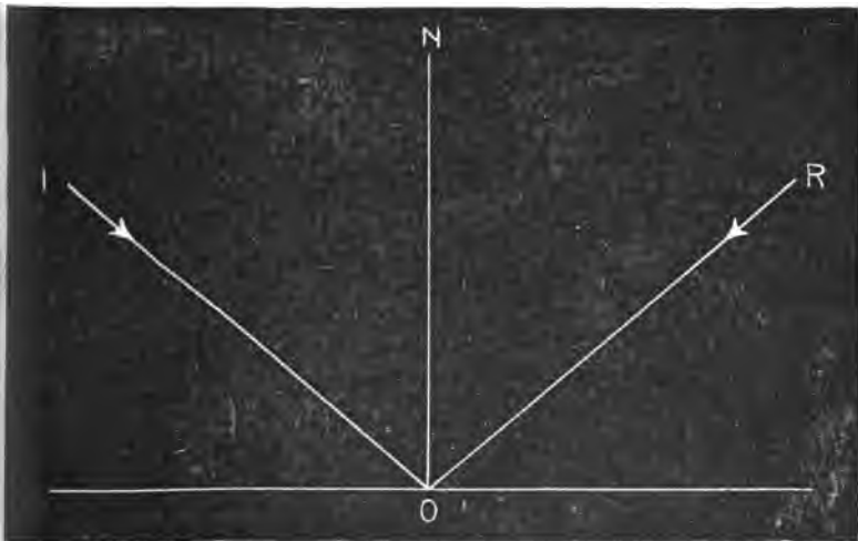
FIG. 3,767. —Angles of incidence and reflection. LAW: the angle of reflection is equal to the angle of incidence. The ray IO is called the incident ray; OR, reflected ray; angle ION, angle of incidence; angle NOR, angle of reflection; NO, normal or perpendicular to the reflecting surface.
