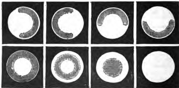
FIGS. 3,869 to 3,876. —Bausch & Lomb diagrams illustrating the results of defective centering, that is, the shadows produced. Successful results in projection depend largely upon the correct adjustment of the lamp, which must throw a brilliantly illuminated circle upon the screen. After the objective is focused, as will be evidenced by a sharp, clear image on the screen, remove slide and slide holder, and examine the illuminated circle. If the light be centered and the lamp correctly adjusted, the circle will be entirely free from coloration or shadows. In figs. 3,869 and 3,870, the crater needs to be properly adjusted laterally, it being as shown too far to the right or left; figs. 3,871 and 3,872, show the crater too high or too low; in figs. 3,873 to 3,875, it is too near or too far from the condenser; fig. 3,876 shows it to be in correct position, the field being entirely clear.
