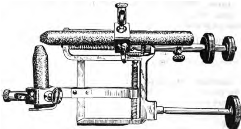
FIG. 3,868. —Ninety degree or right angle arc lamp. With the 90° setting, the arc can be kept nearer in line with the center of the lenses for a greater length of time, without re-adjusting the carbons, because of the horizontal carbon being placed in line with the principal optical axis and fed directly toward the center of the condenser.
