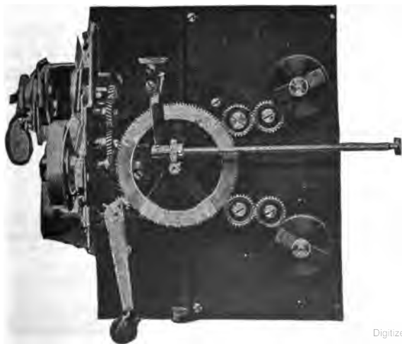
FIGS. 3,893 TO 3,895. —Views of Universal motion picture camera. Fig. 3,893 front view showing lens, fly wheel, shutter, and aperture adjustment; fig. 3,895, right side showing film channel sprocket wheel and shuttle movement. The adjustable shutter may be set for from 25% to 50% exposure. Under ordinary day light conditions and ordinary speed, 37\frac{1}{2}\% (about \frac{1}{8} th second) is found to be the correct time of exposure; fig. 3,894, left side showing arrangement of take up mechanism and stop picture shaft.
