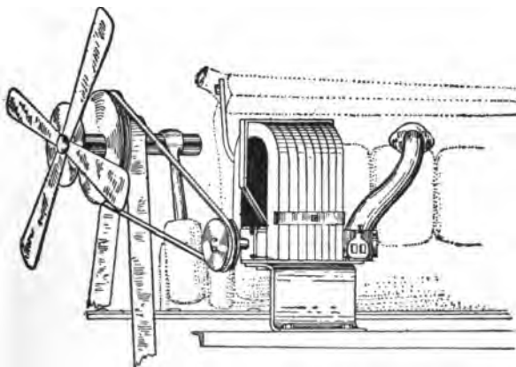
FIG. 4,027. —Holtzer-Cabot lighting magneto as installed on model T Ford car. It must be driven from the fan pulley. A special fan with magneto pulley is furnished with the magneto. The battery is mounted under rear seat on right side; the usual running board mounting is not recommended. A 60 ampere hour storage battery, if fully charged, will operate the side and tail lamps (6 candle power total) for approximately 50 hours, or the head and tail lamps (34 candle power) for approximately 10 hours. Turn off head lights when car is standing.
