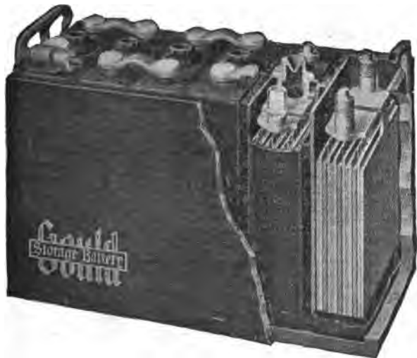
FIG. 4,023 —Gould type B storage battery for starting and lighting systems. Plates 4\frac{1}{4} \times 5\frac{1}{2} ; 7 to 15 plates per cell. Battery units for 6, 8, 12, 16, 18 and 24 volts.
