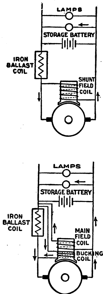
FIGS. 4,051. to 4,053.—Thermal method of obtaining self-regulation in the Rushmore lighting system. As a current of constant volume is desired, it follows that self-regulation must be produced by change in the voltage. The first clue to the solution of the problem was found in a peculiar property by iron, of increasing greatly in electrical resistance at a certain critical temperature just below the red heat. Below this "critical" point the resistance is practically constant. At and beyond the critical temperature, the resistance increases enormously with each degree of temperature increase. Starting from this peculiar property of iron, the next thing was to employ it correctly. The primitive method would have been to insert a thin coil of iron wire directly in the circuit and simply waste the surplus energy at higher speeds in heat as shown in fig. 4,051. This however, would have given very imperfect regulation, besides necessitating a heavy and clumsy machine, since the shunt field winding would receive the full voltage normal to the speed at any moment. To keep down the strength of the current in the
