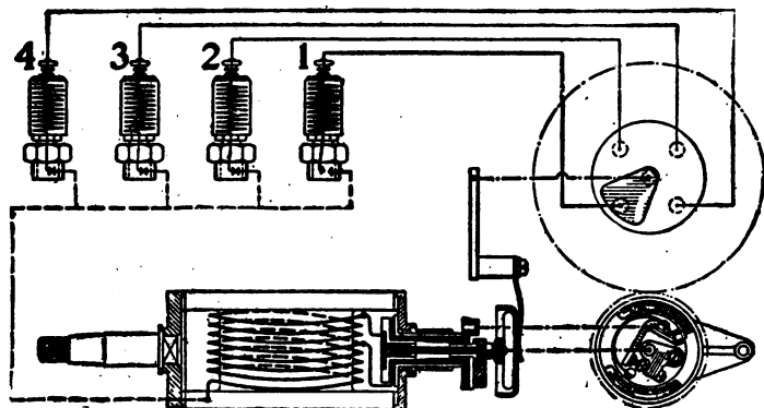
FIG. 3,972. —Wiring diagram of a low tension system with magnetic spark plugs. A portion of the wiring of the magneto armature is short circuited by the platinum points of the interrupter, and when the circuit is broken the resulting armature reaction has the effect of raising the armature voltage sufficiently to operate the plugs.
