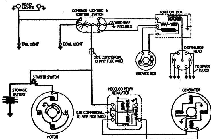
FIG. 2,953.—Wiring diagram of Remy ignition, lighting and starting system as installed on Oakland automobiles. The 6 volt dynamo is a four pole shunt wound machine driven at 1\frac{1}{2} crank speed. A discriminating cut out controls its connection with the battery in charging. The ignition distributor which is a part of the dynamo distributes the high tension current to the cylinders in proper sequence. The interrupter contact points are made of silver.
