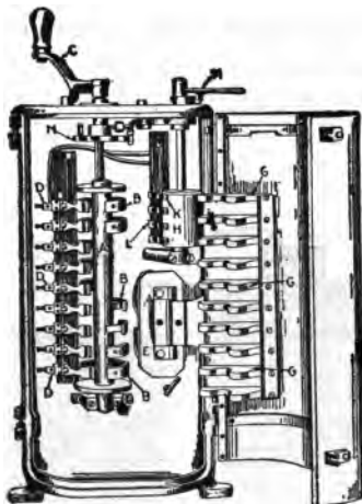
FIG. 3,548. —Ordinary rheostatic controller, designed to control one or more motors by means of resistance only. As shown, it consists of a switch cylinder A, carrying nine insulating supports upon which are mounted nine metallic conducting segments B, B, B. These segments differ in length and position, and when the cylinder is turned by means of the handle C, they come in contact at different times with the nine fixed contact springs D, D, D, which effect the changes in the connection by which more or less resistance is brought into or out of the motor circuit, thereby producing a change in the speed of the car. It is evident that after contact has been made between the motor and the trolley, an electric arc, very destructive to the breaking contact within the controller would be established unless some means were provided for breaking the arc at the instant of its formation. This is accomplished by means of a magnetic blow out device consisting of the magnet E and its pole piece, carrying the polar ridges G, G, G, which rest close to the contact springs D, D, D, when the pole pieces are placed in normal position. In operation, the current passing through the motor passes through the coils of the magnet E, and converts its core into an electromagnet which produces a powerful magnetic flux around the contact surfaces of the springs D, D, D. At the instant the circuit is broken either in changing connections or when the current is entirely shut off, the irresistible influence of this powerful magnetic flux prevents the severe sparking which would naturally occur otherwise by blowing out the arcs as soon as they are formed. The reversing cylinder H, carries four conducting segments K, and a corresponding number of contact spring L. By moving the handle M through an arc of about 60 degrees, the segments in contact with the springs L, can be changed and the direction of the current through the armature of the motor reversed, thereby causing it to rotate in the opposite direction and back the car. As the reversing operation cannot be safely accomplished while the motor is running, the handles C and M are made interlocking so that the latter cannot be moved unless the former be in the "off position." In other words the current must first be shut off before the direction of the car can be reversed. This prevents any arcing on the contacts of the reversing cylinder. The proper operation of a controller requires that all the successive contacts be made and none omitted. This is insured by the action of the star wheel located at N. Rheostatic controllers may be used for single motor railway equipments, single or double motor mining equipments, and for crane, etc. It is important to have a full knowledge of all the requirements of any particular service before selecting the controller. For service requiring frequent motor reversals, a controller with a single handle, with the motor circuits so arranged as to perform the function of the reverser, is found more convenient than a controller with a separate reversing handle. Controllers with single handles are usually employed to operate travelling cranes, turn tables, stationary and portable hoists, etc., while those having two handles are generally used with street railway and mining equipments.
