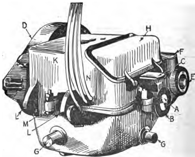
FIG. 3,514. —Direct current railway motor, casing closed as shown, the armature shaft A, projects through its bearing B, lubricated by the grease box C, and is connected with the car axle by gear wheels enclosed in the gear cover D. The gears serve to reduce the speed of the car, and also to increase the effective pull of the motor. The car axle passes through the bearing E, lubricated by the grease box F. The motor is supported on the truck by the lugs G G. The commutator door H gives access to the brushes, while a more complete inspection of the working parts may be obtained by throwing back the upper half of the casing K upon the hinges L L, after unscrewing two bolts, one of which is shown at M. The insulated cables shown at N, pass through the casing and supply current to the motor.
