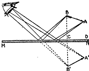
FIGS. 3,763 and 3,764. —Formation of images by plane mirrors. The determination of the position and size of image resolves itself into investigating the images of a series of points. CASE I. Single point A placed in front of a plane mirror , as in fig. 3,763. Any ray AB, incident from this point on the mirror is reflected in the direction BO, making the angle of reflection DBO equal to the angle of incidence DBA. If a perpendicular AN, be let fall from the point A over the mirror, and if the ray OB, be prolonged below the mirror until it meets this perpendicular in the point A', two triangles are formed, ABN and BNA', which are equal, for they have the side BN common to both, and the angles ANB, ABN, equal to the angles A'NB, A'BN; for the angles ANB and A'NB are right angles, and the angles ABN and A'BN are each equal to the angle OBM. From the equality of these triangles, it follows that A'N is equal to AN; that is, that any ray AB, takes such a direction after being reflected, that its prolongation below the mirror cuts the perpendicular AA' in the point A', which is at the same distance from the mirror as the point A. This applies also to the case of any other ray from the point A, as AC. It follows, that all rays from the point A, reflected from the mirror, follow after reflection, the same direction as if they had all proceeded from the point A'. The eye is deceived, and sees the point A at A', as if it were really situated at A'. Hence, in plane mirrors, the image of any point is formed behind the mirror at a distance equal to that of the given point, and on the perpendicular let fall from this point on the mirror. CASE II: Object AB placed in front of the mirror , as in fig. 3,764. The image of any object will be obtained by constructing the image of each of its points, or at least, of those which are sufficient to determine its form. Fig. 3,764 shows how the image A'B' of any object AB is formed.
