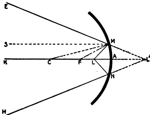
FIG. 3,789.—The virtual focus. If a source of light be placed at L, between the principal focus F, and the mirror, any ray LM emitted from L, makes with the normal CM, an angle of incidence LMC, greater than FMC. The angle of reflection must be greater than CMS, and therefore the reflected ray ME diverges from the axis AK. This is also the case with all rays from the point L, and hence these rays do not intersect, thus forming no conjugate focus. If they be regarded as being prolonged on the other side of the mirror, their prolongations will intersect in a point L', on the axis, giving the same effect to the eye as though the rays were emitted from the point L', this point being called the virtual focus .
