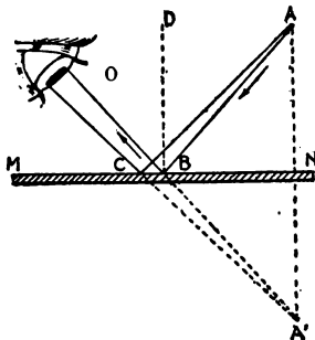
FIGS. 3,763 and 3,764. —Formation of images by plane mirrors. The determination of the position and size of image resolves itself into investigating the images of a series of points. CASE I. Single point A placed in front of a plane mirror , as in fig. 3,763. Any ray AB, incident from this point on the mirror is reflected in the direction BO, making the angle of reflection DBO equal to the angle of incidence DBA. If a perpendicular AN, be let fall from the point A over the mirror, and if the ray OB, be prolonged below the mirror until it meets this perpendicular in the point A', two triangles are formed, ABN and BNA', which are equal, for they have the side BN common to both, and the angles ANB, ABN, equal to the angles A'NB, A'BN; for the angles ANB and A'NB are right angles, and the angles ABN and A'BN are each equal to the angle OBM. From the equality of these triangles, it follows that A'N is equal to AN; that is, that any ray AB, takes such a direction after being reflected, that its prolongation below the mirror cuts the perpendicular AA' in the point A', which is at the same distance from the mirror as the point A. This applies also to the case of any other ray from the point A, as AC. It follows, that all rays from the point A, reflected from the mirror, follow after reflection, the same direction as if they had all proceeded from the point A'. The eye is deceived, and sees the point A at A', as if it were really situated at A'. Hence, in plane mirrors, the image of any point is formed behind the mirror at a distance equal to that of the given point, and on the perpendicular let fall from this point on the mirror. CASE II: Object AB placed in front of the mirror , as in fig. 3,764. The image of any object will be obtained by constructing the image of each of its points, or at least, of those which are sufficient to determine its form. Fig. 3,764 shows how the image A'B' of any object AB is formed.
