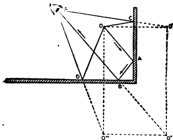
FIG. 3,768.—Multi-image formed by two mirrors. When an object is placed between two plane mirrors, which form an angle with each other, either right or acute, images of the object are formed, the number of which increases with the inclination of the mirrors. If they be at right angles to each other, three images are seen, arranged as represented in the figure. The rays OC and OD from the point O, after a single reflection, give the one, an image O' , and the other an image O'' , while the ray OA, which has undergone two reflections at A and B, gives the third image O''' . When the angle of the mirror is 60^\circ , five images are produced, and seven if it be 45^\circ . The number of image continues to increase in proportion as the angle diminishes, and when it is zero (mirrors parallel), the number of image is infinite. In general , if two mirrors be inclined to each other, the number of image they produce is equal to the number of times the angle between them is contained in 360 .
