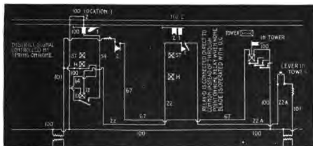
FIG. 3,739. —Distant signal and repeater circuit. Here, through a lever connection, when the lever is pulled out in the tower, current is allowed to flow to and complete a circuit through a contact spring operated by the signal mechanism. As soon as the distant blade clears, according to this circuit, a repeater located in the tower is de-energized and drops its armature, which shows the position of the blade whose action governs its source of energy.
