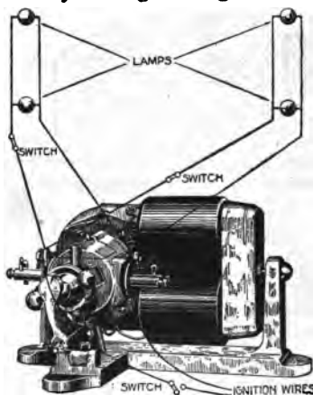
FIG. 3,952.—Motsinger "Auto Sparker" friction drive dynamo. The small friction pulley gives sufficient speed to ignite the charge when engine is turned slowly as in cranking. After the engine is under motion, the governor on the shaft of the dynamo limits its speed so as not to obtain an excessive voltage. This is accomplished by mounting the dynamo on its base so that it can oscillate on an axis, the small friction wheel making and breaking contact with the engine fly wheel. In operation , when normal speed is exceeded, the governor weights fly out and draw the friction wheel away from the fly wheel, one spring serving the double purpose of pushing the friction pulley against the fly wheel and acting as a tension on the governor. By increasing or diminishing the tension on the governor spring by means of a thumb nut provided for the purpose, the speed of the dynamo may be increased or diminished, which in turn increases or diminishes the volume of current and size of spark. By screwing up on this thumb nut the position of the dynamo is not changed, but the contact of the pulley and tension of the governor are increased. Thus, by adjusting the thumb nut, the size of the spark may be regulated at will.
