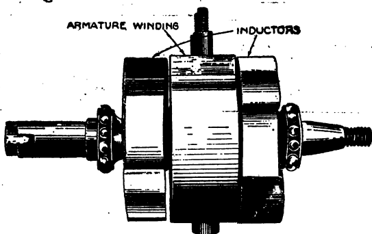
FIG. 3,954. —Remy ball bearing shaft showing inductors and stationary armature of inductor magneto. This type of magneto consists of a winding which is held stationary between the pole pieces, on either side of which revolves a laminated steel inductor . Inasmuch as the winding is held rigidly stationary, such construction eliminates all revolving or moving wires, all sliding or wiping contacts, collector rings, etc. This design permits of rugged electrical, as well as mechanical, construction. In operation , at each half turn of the inductor shaft, the direction of flow of the lines of force through the winding is reversed, producing in the winding two electrical impulses for each complete revolution. The stationary winding is directly connected through the magneto circuit breaker with the primary of the secondary coil used with the magneto. The timing of the spark is accomplished by shifting the circuit breaker around the inductor shaft, to which is attached the circuit breaker cam. The timing range is 35 degrees.
