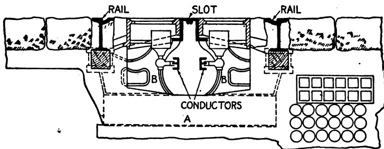
FIG. 3,513. —Sectional view showing construction details of conduit system of the Third Ave. Street Railway, New York City. A 4 inch layer of concrete forms a surface on which to align the iron work, all of which is assembled before the main body of concrete is installed. The track rails and slot rails are supported on iron yokes spaced 3 feet apart and made up in three pieces, which is a new feature in such work. The three members are a steel I beam A and two cast iron side pieces B, weighing about 125 pounds each. The yokes rest on the 4 inch concrete bottom, and the space between the yokes, the center of which space is the conduit proper, is filled with concrete that must be put in after the iron is in place, because the throat of the yoke dictates the general shape of the concrete part of the conduit. In order to shape the walls between the yokes, iron linings are used to support the concrete until it has set. These linings are made so that they can be freely drawn through the slot either way, and they are forced into position by means of a folding form operated by a lever. The track rails are 9 inch grooved girders 107 pounds to the yard, in 60 foot lengths, laid on pine stringers. This stringer construction is in accordance with the idea held by many engineers that a rigid support for the rails does not afford an easy riding track.
