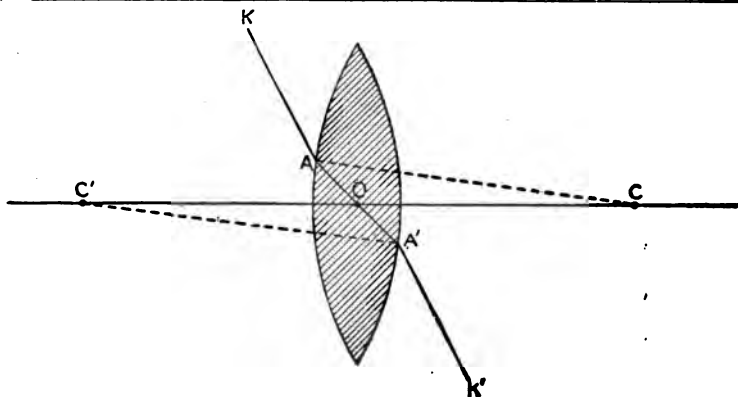
FIG. 3,796.—Optical center. Let two parallel radii of curvature CA and C'A' be drawn to the two surfaces of a double convex lens. Since the two plane elements of the lens A and A' are parallel, as being perpendicular to two parallel right lines, it is evident that the refracted ray AA' is propagated in a medium with parallel faces. Hence a ray KA , which reaches A at such an inclination that after refraction it takes the direction AA' , will emerge parallel to its first direction. The point O at which the right line cuts the axis is therefore the optical center. The position of this point may be determined from the case in which the curvature of the two faces is the same, which is the usual condition, by observing that the triangles COA and C'O'A' are equal, and therefore that OC = OC' , which gives the point O . If the curvatures be unequal, the triangles COA and C'O'A' are similar, and either CO or C'O may be found, and therefore also the point O . In double concave or concavo-convex lenses, the optical center may be determined by the same construction. In lenses with a plane face, this point is at the intersection of the axis by the curved face.
