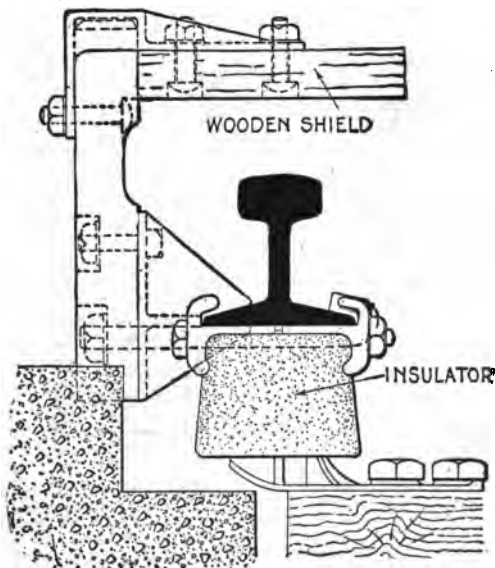
FIG. 3,694.—Cross section showing cartrack of protected top contact third rail.
