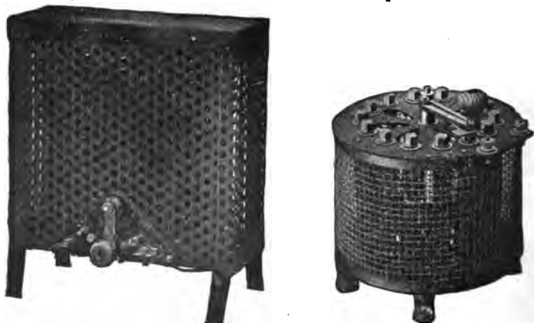
FIGS. 3,879 and 3,880. —Powers' rheostats. The type shown in fig. 3,879 is designed for use on 110 volt circuits and will carry 25 amperes without overheating. The coils are so supported that any of them may be replaced when desired. Adjustment is effected by means of a lever switch. Fig. 3,880 shows Underwriters' pattern rheostat of 25 amperes capacity. It is designed for 110 volts and is not adjustable.
