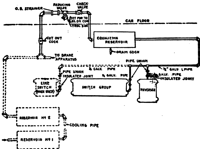
FIG. 3,635. —Arrangement of piping of Westinghouse unit switch control, type HL. The piping here shown is for the compressed air which operates the control apparatus, the air supply being taken from the brake system. The air passes through a cut out cock for shutting off the supply if desired, a hair strainer for removing dirt or scale, and a reducing valve, with equalizing reservoir and check valve for maintaining a uniform pressure. The amount of air required for operating the switches is so small compared to that required by the brakes and whistle that it is practically negligible.
