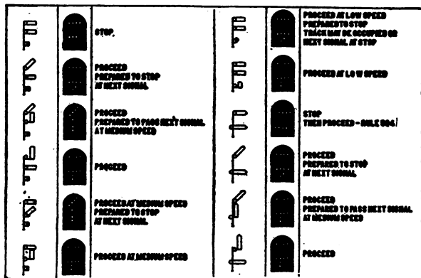
FIG. 3,716. —Corresponding aspects of semaphore and position light signals with their indications. Early in 1914 Dr. Churchill of the Corning Glass Company, while working on some of the electric headlight troubles of the western railroads, discovered that it was possible to secure very long range from a small light source located in the exact focal point of a small wide angle lens, and in talking the matter over with A. H. Rudd, signal engineer of the Pennsylvania, it was seen to be altogether practicable to combine these small separate units into rows of lights which would have the effect of the present semaphore arm and would do away with the color scheme altogether. Thus was evolved the position light signal, which has now been covered by various patent applications. It was, of course, a long way from the conception of the idea to the perfection of the design, and it was not until the summer of 1914 that the signal was considered satisfactory enough to adopt. The principal experiments were conducted at Wayne and later at Paoli.
