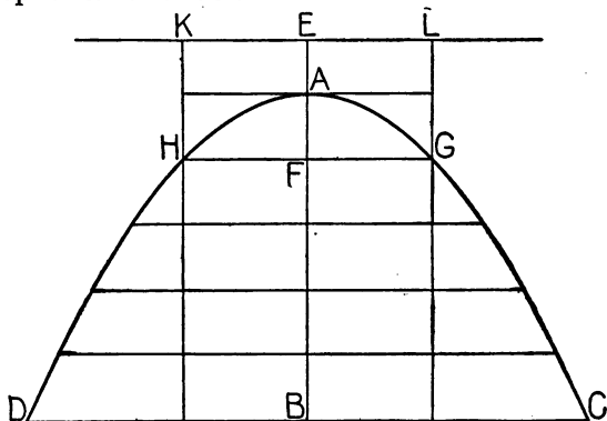
FIG. 3,770. —The parabola. A parabola DAC is a curve such that every point in the curve is equally distant from the directrix KL and the focus F. The focus lies in the axis AB, drawn from the vertex or head of the curve A, so as to divide the figure into two equal parts. The vertex A, is equidistant from the directrix and the focus or AE = AF . Any line parallel to the axis is a diameter. A straight line, as HG or DC, drawn across the figure at right angles to the axis is a double ordinate, and either half of it is an ordinate. The ordinate to the axis HFG drawn through the focus, is called the parameter of the axis. A segment of the axis, reckoned from the vertex, is an abscissa of the axis, and it is an abscissa of the ordinate drawn from the base of the abscissa. Thus AB is an abscissa of the ordinate BC. Abscissae of a parabola are as the square of their ordinates.
