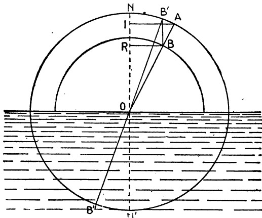
FIG. 3,776. —Construction of refracted ray. Let AO be a ray of light passing through air and entering water at O. The index is \frac{4}{3} . Draw two circles with centers at O and with radii whose lengths are as 4 : 3. Draw AI and BR perpendicular to the normal NN'. Since AO : BO = 4 : 3, then AI : BR = 4 : 3. Hence if AI be the sine of the angle of incidence, BR is the sine of the angle of refraction. If then, BB' be drawn parallel to the normal, and a straight ruler be placed on the points B' and O, the line OB', the refracted ray may be drawn.
