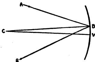
FIGS. 3,771 and 3,772.—Concave spherical mirror; definitions. In the diagram V is the vertex; MM', the aperture; CV, the principal axis; CS, a secondary axis; C, center of curvature; F, principal focus (midway between V and C). Any line drawn from C to the mirror will be perpendicular to the mirror at that point. This line then will always be the normal which will be used in making the angle of incidence equal to the angle of reflection. Now in fig. 3,772, if AB be an incident ray of light, the angle ABC is the angle of incidence . To find the direction of the reflected ray draw BR so that the angle CBR equals angle ABC, then will BR be the direction of the reflected ray.
