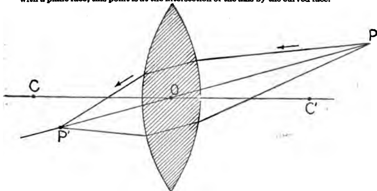
FIG. 3,797.—Secondary axis. This is any right line passing through the optical center, but not through the centers of curvature. Rays emitted from a point P on the secondary axis PP' nearly converge to a center point P' on the axis PP' , and according as the distance from the point P to the lens is greater or less than the principal focal distance, the focus thus formed will be conjugate or virtual. The formation of image is in accordance with this principle.
