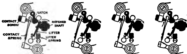
FIGS. 4,001 to 4,004.—Principle of the Atwater-Kent ignition system. The so called "uni-sparker" consists of a notched shaft, one notch for each cylinder, which rotates at one-half the engine speed, a lifter or trigger which is pulled forward by the rotation of the shaft and a spring which pulls the lifter back to its original position. A hardened steel latch and a pair of contact points complete the device. The figures show the operation of the contact maker very clearly. It will be noted that in fig. 4,001 the lifter is being pulled forward by the notched shaft. When pulled forward as far as the shaft will carry it fig. 4,002, the lifter is suddenly pulled back by the recoil of the lifter spring. In returning, it strikes against the latch, throwing this against the contact spring and closing the contact for a very brief instant—too quickly for the eye to follow the movement (fig. 4,003). Fig 4,004 shows the lifter ready to be pulled forward by the next notch. Note that the circuit is closed only an instant preceding the spark. No current can flow at any other time, not even if the switch be left "On" when the engine is not running. Note that no matter how slow or how fast the shaft is turning, the lifter spring will always pull the lifter back at exactly the same speed, so that the operation of the contact, and therefore the spark, will always be the same, no matter how fast or how slow the engine be running. The contact points are adjustable only for normal wear. By means of the distributor, which forms the upper part of the uni-sparker, the high tension current from the coil is conveyed by the rotating distributor block, which seats on the end of the uni-sparker, to each of the four spark plug terminals in the order of firing.
