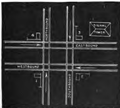
FIG. 3.742. —Intersection of two double track lines, with their respective signals. If these be automatic track relays properly interconnected, they can be readily arranged to give the protection desired. If they be semi-automatic, electric interlocking will be introduced to prevent conflict of routes. Thus, when signal 3 is at clear, to allow a south bound train to pass, 2, and 4, must be locked in the normal or stop position when electric locking or interlocking is used and prevented moving to clear if the ordinary automatic system be employed.
