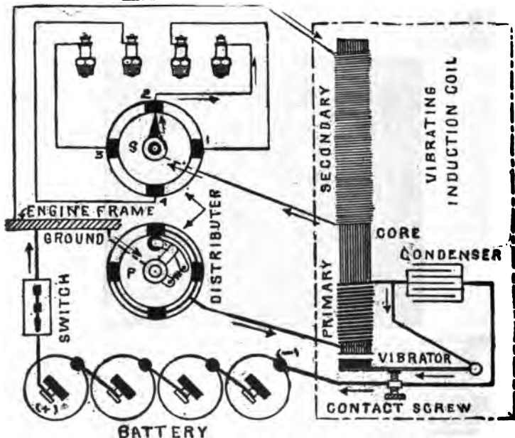
FIG. 3,998. —Diagram illustrating the principles of synchronous ignition. For clearness the primary and secondary elements of both the coil and the distributor are shown separated. When the primary rotor of the distributor completes the primary circuit, current from the battery flows and the vibrator operates, making and breaking the current with great frequency. A high tension current, made up of a series of impulses, is induced in the secondary circuit and distributed by the rotor arm during its revolution to the several cylinders in the proper order of firing. Each secondary segment of the distributor being wired to one of the spark plugs, the rotor during its revolution brings each plug into the secondary circuit in the order indicated in the diagram. As shown, the secondary rotor is in contact with segment number two which causes the induced current to flow from the secondary winding, through the distributor. One end of the secondary winding is usually connected to one end of the primary winding instead of making a separate ground connection to the metal of the engine. This simplifies the wiring by having one common ground connection.
