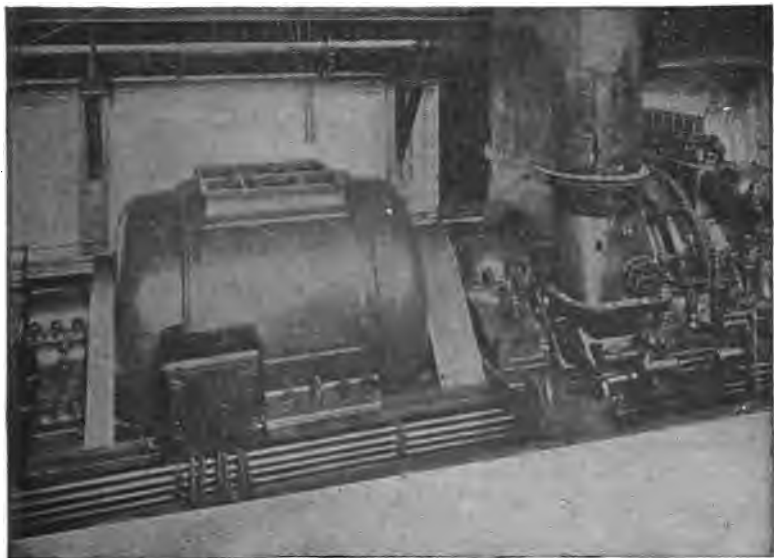
FIG. 3,759.—Generating unit of U. S. Collier Jupiter, consisting of an alternator directly connected to a turbine.
