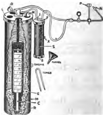
FIGS. 3,862 to 3,865. —The Economic calcium light; makes its own gas automatically from oxone and ether. Fig. 3,863 shows section view of interior of outfit. The parts are: M, main tank; L, cover for tank; G, gas bell or chamber; C, container for holding charge of oxone; R, wire rod for supporting container in position; O, needle valve controlling flow of oxygen gas direct to burner; H, needle valve controlling flow of gas through saturator S which causes ether vapor (hydro-carbon gas) to flow to burner; S, saturator; I, inlet connecting with nipple of needle valve H; F, filler plug; X, overflow; B, bottom cap of saturator; P, pastil; N, nozzle of burner.
