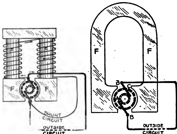
FIGS. 3,949 and 3,950.—Circuit diagrams to illustrate the difference between a dynamo and a magneto. The former has its field magnets FF magnetized by means of a small current flowing around a shunt circuit. In a magneto the field magnets are permanently magnetized. The strength of the magnetic field of a magneto is constant while that of a dynamo varies with the output, hence, a magneto may be run at a widely varying speed and meet ignition requirements, but a dynamo must have its speed maintained approximately constant to keep the voltage within limits.
