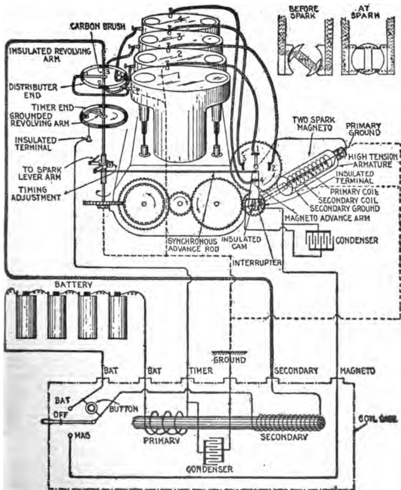
FIGS. 3,955 to 3,957. —Double ignition consisting of a two spark high tension magneto system, and a battery synchronous ignition system with engine driven distributor. Fig. 3,955 elementary diagram of connections; fig. 3,956, position of magneto armature just before time of spark; fig. 3,957, position of armature at time of spark.
