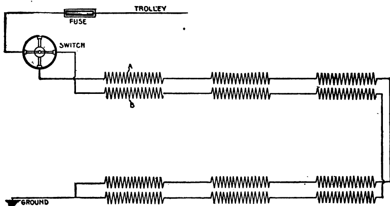
FIG. 3,682.—Wiring diagram of six heater equipment with type of heater shown in fig. 3,682. Three variations in the amount of heat furnished may be obtained with this arrangement, a suitable switch being provided by means of which either the smaller, or the larger coils (see fig. 3,682), or all the heaters may be turned on at a time, or both sets of coil may be operated at the same time.
