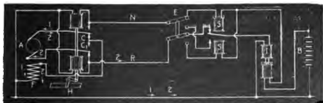
FIG. 3,740. —Diagram illustrating electric interlocking. A switch and lock movement is driven by a direct current motor, the shaft of which is connected by a magnetic clutch to an extension working a cam drum which operates the switch and lock. When the drum is revolved by the motor, first the lock rod and then the switch move in proper operation. After the switch has been moved against the stock rail it is automatically locked and a knife switch throws open the control circuits and closes the indication circuit. The direction of rotation for reversing the switch is controlled by a double field winding in the motor, one part of which is cut out while the other is in circuit.
