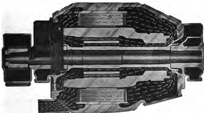
FIG. 3,519. —Method of forced ventilation with external air. In construction , the fan is cast integral with the pinion end armature head, which draws air in through a screened inlet. In operation , the air passes around field coils, over and through the commutator and armature coil, carrying the heat from the interior, and thus increasing the service capacity of the motor.
