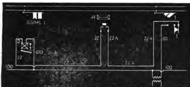
FIG. 3,738. —Advanced block distant signal. In operation when the towerman pulls a lever numbered the same as the distant signal he desires to operate, he completes a circuit between the two springs which causes the distant signal blade to clear.
