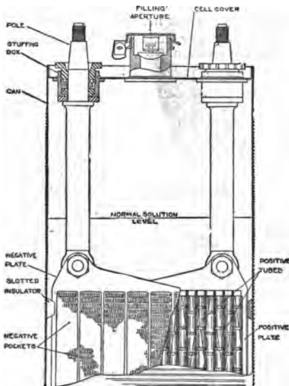
FIG. 3,948.—Sectional view showing construction of Edison cell. The solution should be maintained 2\frac{3}{4} inches above plates. If solution level be low in any cell, hold battery out of service until renewal solution can be obtained. Normal charge. After battery has been practically discharged, the normal charge is for seven hours at normal rate. Charging resistance should be adjusted from time to time to keep current normal. If this be impracticable, set resistance so that current is about 50 per cent. above normal at the start. It should taper off by rise in battery voltage so that the average current will be at normal rate. If battery be only half discharged, recharge for half of seven hours at normal rate; if only one quarter discharged, charge for a quarter of seven hours, etc. Low rate charge. To secure best results on five hour or eight hour discharge, charge at not less than the normal rate. If, however, the cells be discharged at a very low rate, a charging rate lower than normal can be used with satisfactory results. Ampere hour meter. An ampere hour meter, if used, should be set to recharge 25 per cent. in excess of discharge. Discharge rate. The size of cell used should be such that the continuous discharge does not exceed 25 per cent. above normal rate. Water. Replenish cells with distilled water as frequently as is necessary to keep solution level above tops of plate. When adding water do so before charging. Changing solution. After about every nine or ten months of continuous daily service, test solution with hydrometer after a full charge. If it read below about 1.160, the solution should be changed.
