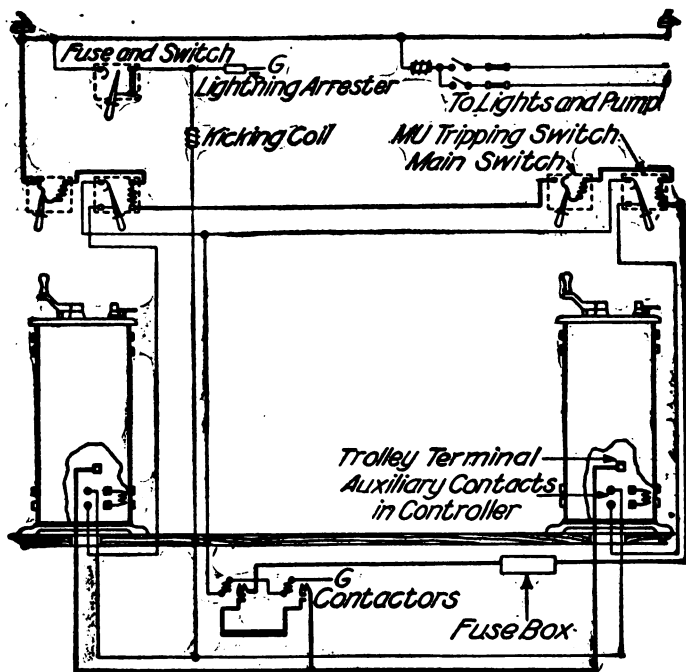
FIG. 3,581. —Wiring diagram of General Electric contactor equipment, designed to eliminate all destructive arcing from the car platform, by opening and closing the main power circuit with contactors located underneath the car body. Two of these contactors are connected in series in the main circuit between the trolley base and the controller and are enclosed in an iron box for protection. Additional contacts are provided in the controller for opening and closing the operating circuit of the contactors when the controller is turned off or on respectively. By this arrangement heavy arcing is avoided at the controller. This equipment also includes overload devices, tripping switches for interrupting the energizing circuit of the contactor coils in case of overload. These switches perform the function of the circuit breakers ordinarily used, and are located in the cab convenient for operation by the motorman. They are adjusted, set and tripped the same as a circuit breaker but only open the small energizing current of the contact coils. A combined switch and fuse is connected in the contactor operating coil circuit. Where the auxiliary contactor equipment is used, the car circuit breakers are usually replaced with non-automatic magnetic blowout switches, for opening the main circuit when desired.
