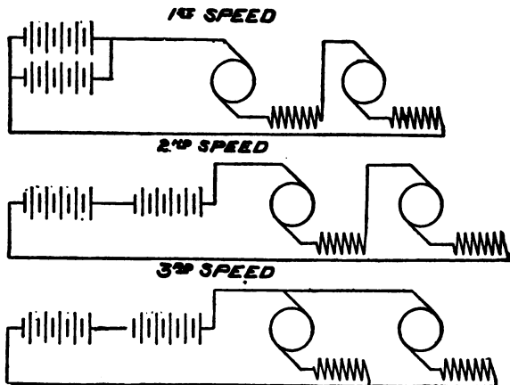
FIGS. 4,102 to 4,104. —Diagram showing methods of speed changing in a two battery unit, two motor circuit, showing combinations for three speeds. The first speed is obtained with the battery units in parallel, and the motors in series; the second , with the battery units in series and the motors in series; the third , with the battery units in series and the motors in parallel.
