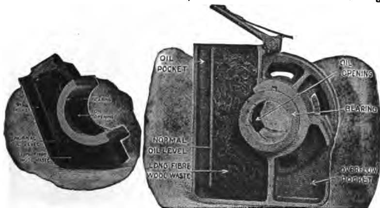
FIGS. 3,656 and 3,657. —Westinghouse self-lubricating bearing. Fig. 3,656 type used on box frame motor; fig. 3,657 type used on split frame motor. As shown in the sectional views, the bearing housing has a separate oil pocket from which the oil is fed and which may, at any time, be gauged. With this arrangement there is no excuse for wasting oil. The inspector pours only enough oil into the chamber to bring the free oil up to a predetermined depth. With the supply of free oil normally below the level of the opening in the bearing there is no oil wasted when the motors are at rest through dripping or draining. The bearing is provided with suitable wiper rings, that prevent an over supply of oil working into the motor and damaging the windings. In addition, it has an easily accessible drain chamber, that catches the oil as it works out of the bearings. There is no variation in saturation of the waste. In modern Westinghouse motors the armature bearings are lubricated on the low pressure side. With this type of bearing it is usually sufficient to renew the oil once a month.
