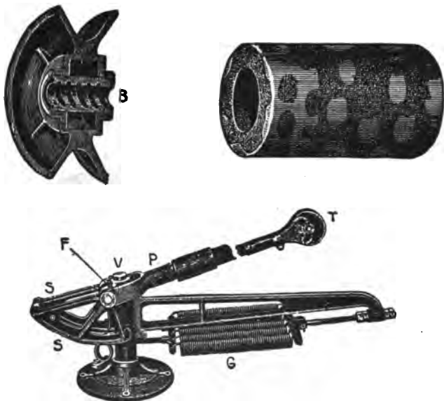
FIGS. 3,503 and 3,504. —Section through trolley showing lubricating bushing, and view of bushing removed from trolley. Since trolleys revolve at a very high speed, some unusual means of lubrication must be provided, as shown in fig. 3,503. The trolley hub is fitted with a brass bushing, having a spiral groove into which is pressed graphite which acts to fill the pores of the metal, thus giving a smooth surface which reduces the friction. Roller bearing wheels have been used to a limited extent with considerable success. On some lines a very long journal is used instead of the usual short brass graphite bushing.
