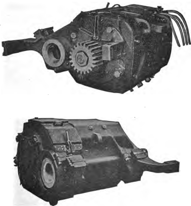
FIGS. 3,751 and 3,752. —Westinghouse interpole motor as used on Piedmont railway. Fig. 3,751 pinion end of motor; fig. 3,752 commutator end. The motor is rated at 110 horse power at 750 volts. Two motors are connected in series for 1,500 volt operation. These motors are geared to 36 inch wheels with a 20 tooth pinion and 57 tooth gear. The cars, weighing complete without load, approximately 41 tons, are operated at a schedule speed of 34 miles per hour. The weight of the motor complete is 4,150 pounds. The armature is especially designed to withstand the higher voltage, being insulated with mica, and having liberal creepage distances provided at the end of the commutator. The brush holders have extra heavy porcelain insulators. The length of the dust ring at the end of the commutator, and the clearances from the line parts of the motor to the ground are greater than in ordinary designs.
