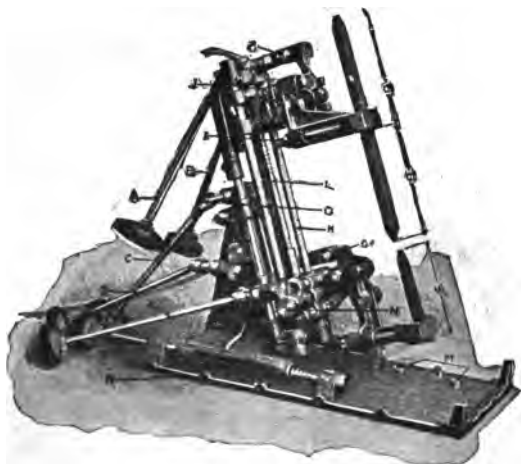
FIG. 3,877. —Simplex arc lamp. The carbon holders are furnished to accommodate carbons of \frac{1}{8} " to \frac{3}{4} " diameter and 12" upper and 6" lower in length, carrying capacity 75 amperes. There are eight adjustments, six being accessible from the back of the lamp house; and two, to alter the angle of the carbon, from the inside. The lamp can be withdrawn from the back of the lamp house, so that all parts are readily accessible.
