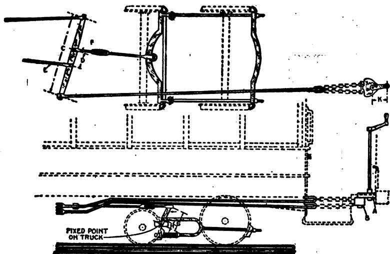
FIG. 8,667. —Geared brake. This apparatus has a pinion A, on the lower end of the brake shaft , which engages a gear B, made in one piece with a double sprocket wheel. The two chain loops running through these sprocket wheels engage two hooks formed on the end of the brake rod, or two separate brake rods which are attached at the same point the sway bar. The upper chain is the only one used in braking, the other being left slack and held in reserve for use if the first set fail to work. When the brake is applied to a car mounted on maximum traction trucks as shown, the difference in pressure between the brake shoes on the driving wheels and those on the pony wheels is obtained by means of a spring interposed between the brake system and the pony wheel brake shoes. The dimensions of the different levers are as follows: Length of sway bar C is 48 inches; distance D between pins for the arch bar rods E and F is 9 inches; length truck lever B is 13 inches; and length of horizontal part of brake handle K is 15 inches. With levers of these dimensions a force of 65 pounds applied at the brake handle gives a total braking pressure of 29,000 pounds, or an amount exceeding the weight of an empty car. The best proportion of the lever is secured when, (C + D) \times (G \times H) \times 85k = \text{total weight of the empty car} .
