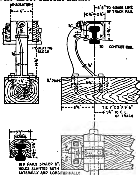
FIGS. 3,509 to 3,512. —Construction details of New York Central Railroad inverted third rail.
