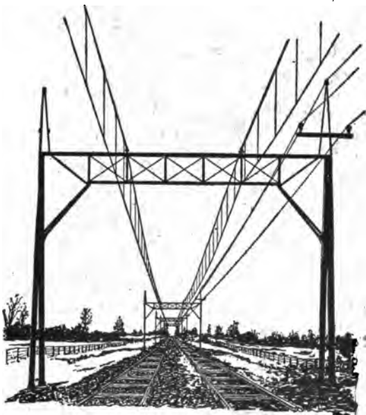
FIG. 3,700. —Bridge type single catenary construction for double track road. In this arrangement the trolley wire is suspended from a messenger cable supported on bridges spanning the tracks and supported by towers on each side. This type of construction is seldom used for anything but the heaviest class of service, such as electrified steam railroads, and substantial interurban roads handling heavy freight traffic as well as heavy passenger traffic.
