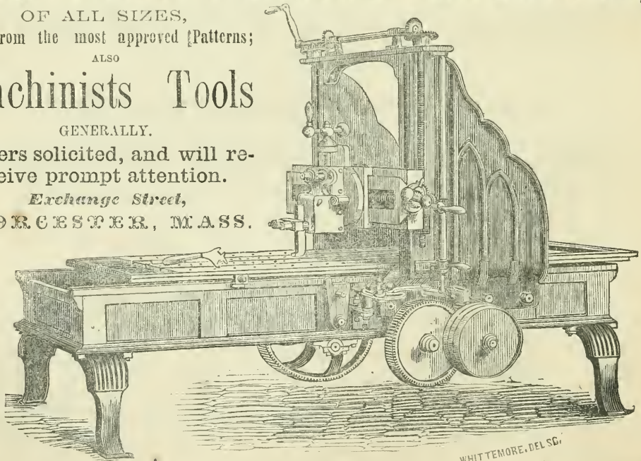
Cut of 8 foot Planer,—Planes 6 1-2 feet long, 24 by 24 Inches.
