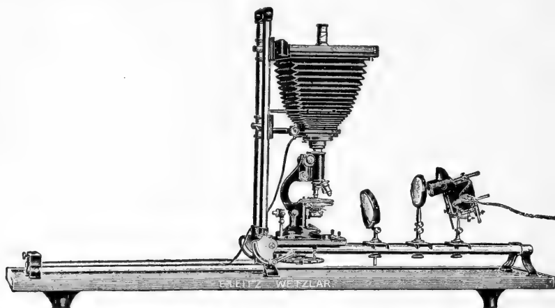
FIG. 29.—Microphotographic Apparatus
