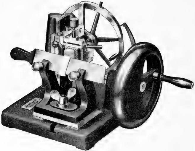
FIG. 37.—Minot Rotary Microtome
