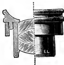
FIG. 9.—Abbé Condenser
