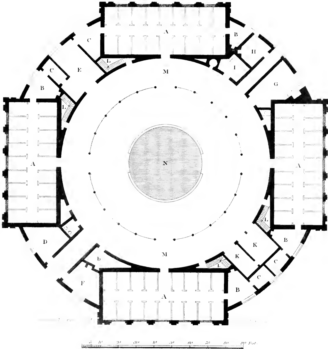
ELEVATION AND GROUND PLAN OF A STABLE.
