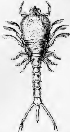
FIG. 26.— Diastylis Goodsiri , dorsal view of female [Hansen].
