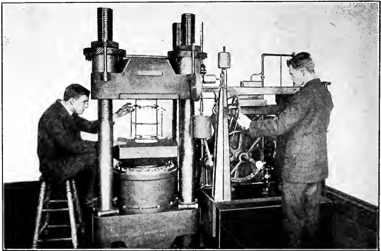
Compression Machine. Capacity, 1,200,000 Pounds
