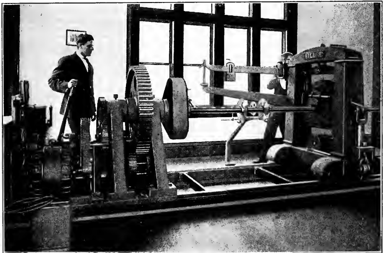
Torsion Machine. Capacity, 125,000 Inch Pounds
