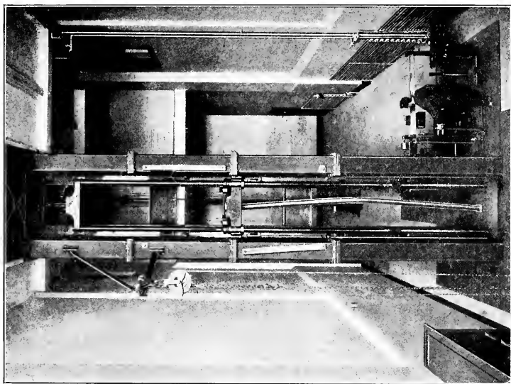
Testing Machine. Capacity, 600,000 Pounds
