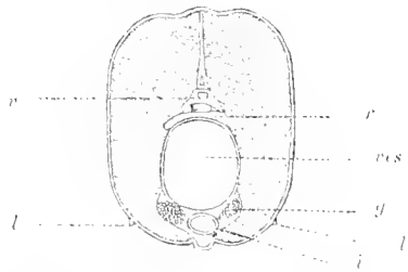
Fig. 96. Transverse section of a Flying-fish: v , vertebræ; r , kidneys; ves , air-bladder; g , organs of generation; l , lateral lines; i , intestine. After MÖBIUS.
