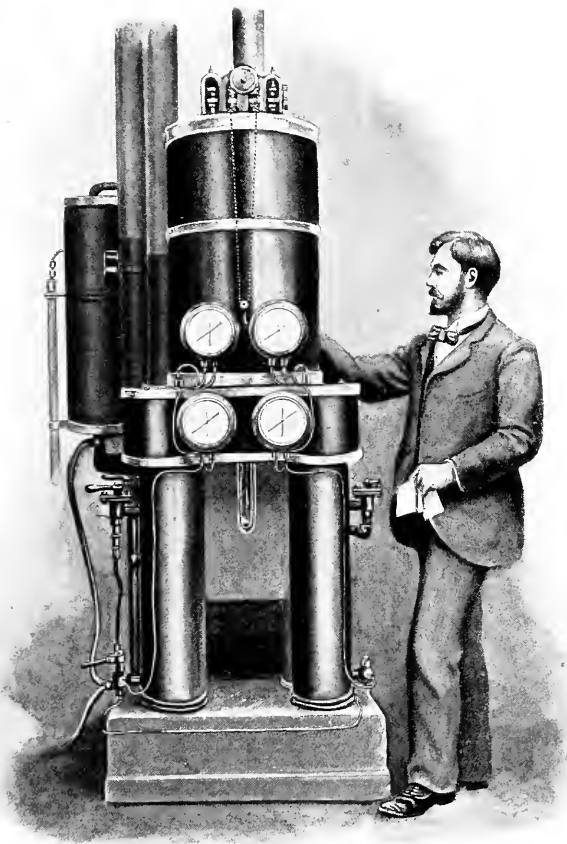
PROFESSOR DEWAR'S APPARATUS WITH WHICH HYDROGEN WAS FIRST LIQUEFIED
