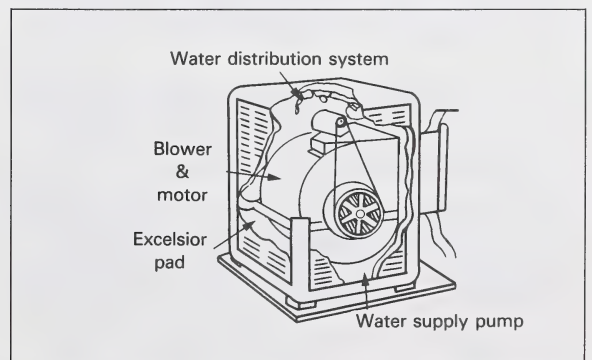
Figure 29. Arctic cooler
