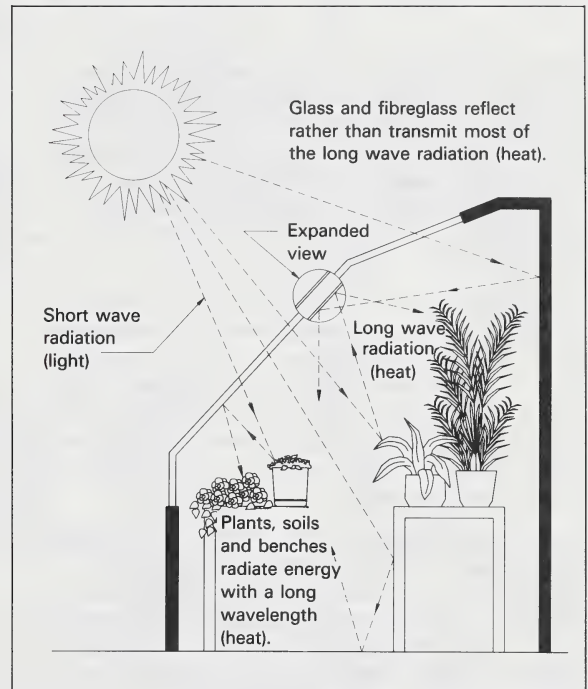
Figure 12. The greenhouse effect
