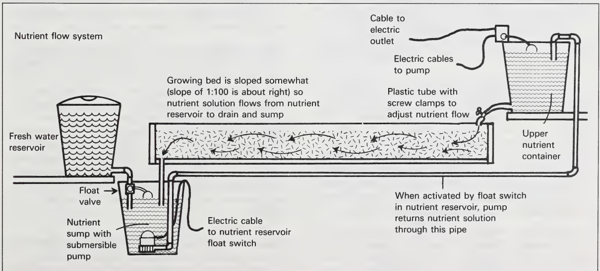
Figure 37. An automatic hydroponic garden
