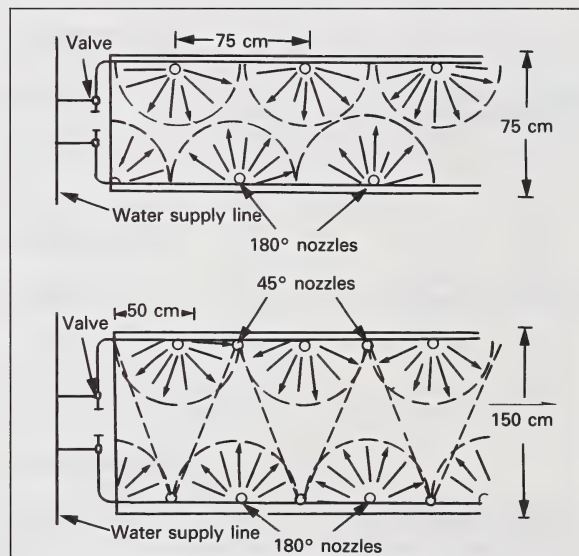
Figure 33. Mist nozzle watering system
