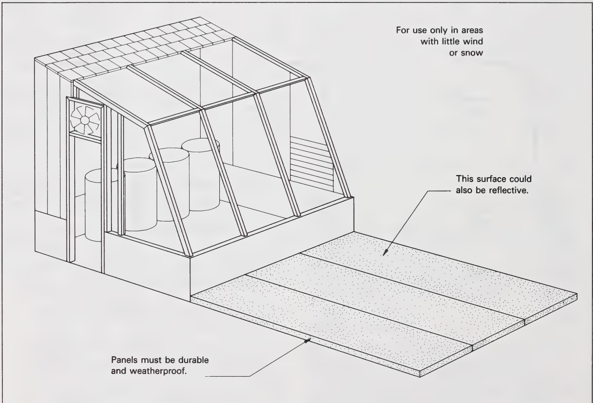
Figure 23. Exterior insulation system
