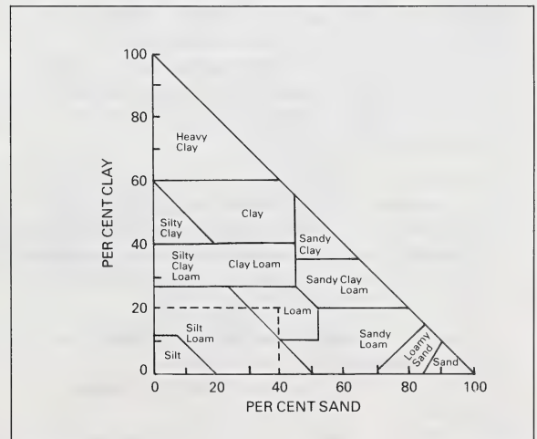
Figure 35. Soil texture triangle
