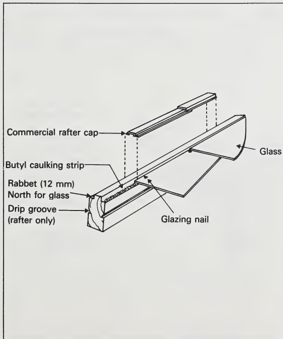
Figure 13. Installation of glass in the greenhouse
