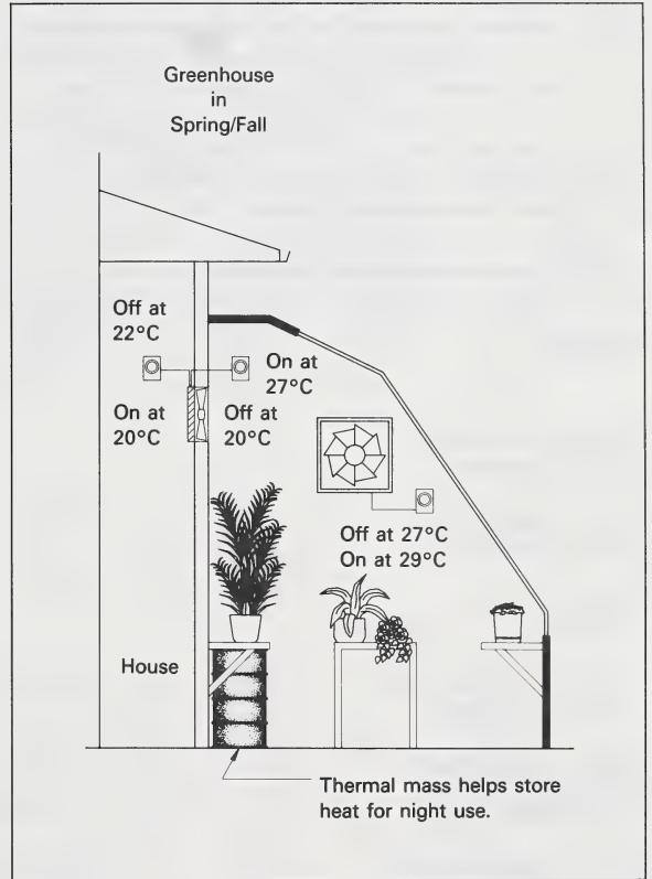
Figure 20. Heating an attached greenhouse from the house
