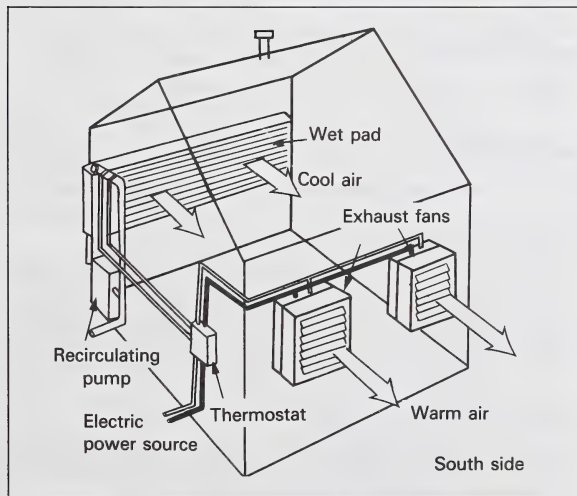
Figure 28. Pad and fan cooling systems
