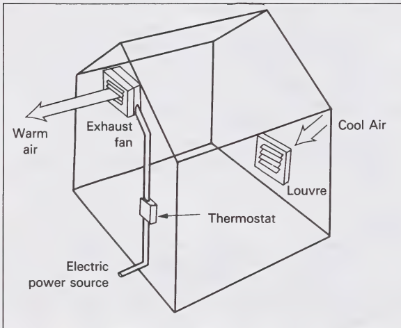
Figure 26. Ventilation by fans
