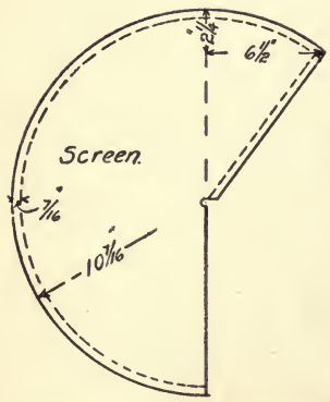
PATTERN OF INSIDE CONE
