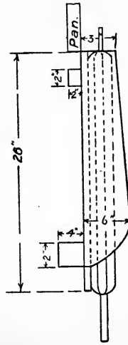
Butter Worker.
