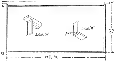
FIG. 24.—Langstroth frame; size, 17\frac{7}{8} in. by 9\frac{7}{8} in. outside; pn , projecting nail. (Original.)
