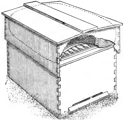
FIG. 26.—Lock-joint chaff hive. (From Gleanings in Bee Culture.)
