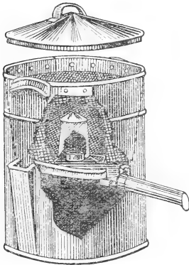
FIG. 36.—Excelsior wax extractor.
