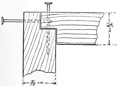
FIG. 27.—Manner of nailing hives. (Original.)
