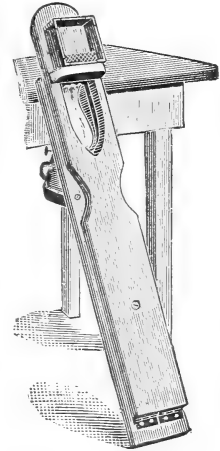
FIG. 40.—The Daisy foundation fastener. (From Gleanings.)
