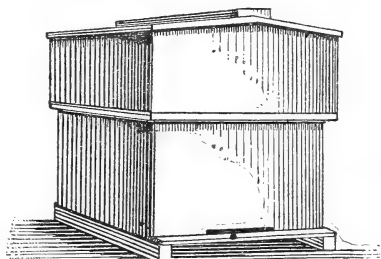
FIG. 74.—Double-walled hive adapted to outdoor wintering as well as summer use below 40^{\circ} north latitude in the United States. Thickness of each wall, \frac{3}{8} inch; space between walls, 2 inches, packed with dry chaff or ground cork. (Original.)
