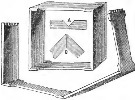
FIG. 56.—One-piece V-grooved sections. (From Gleanings.)
