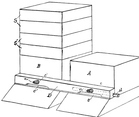
FIG. 70.—Beehives with Langdon non-swarmers attached: A, B , hives; S, S' , supers; D , non-swarming device; e, e' , entrances corresponding to hive entrances; sl , slide for closing entrance; c, c' , conical wire-cloth bee-escapes; ex, ex' , exits of same. (From Insect Life .)
