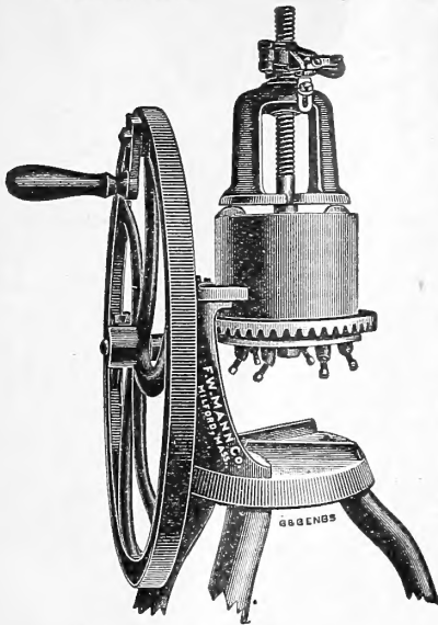
Mann's No. 4 Green Bone Cutter.
