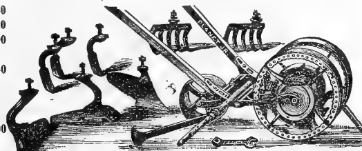
THE "PLANET, JR." NO. 1 COMBINED DRILL AND WHEEL HOE.
