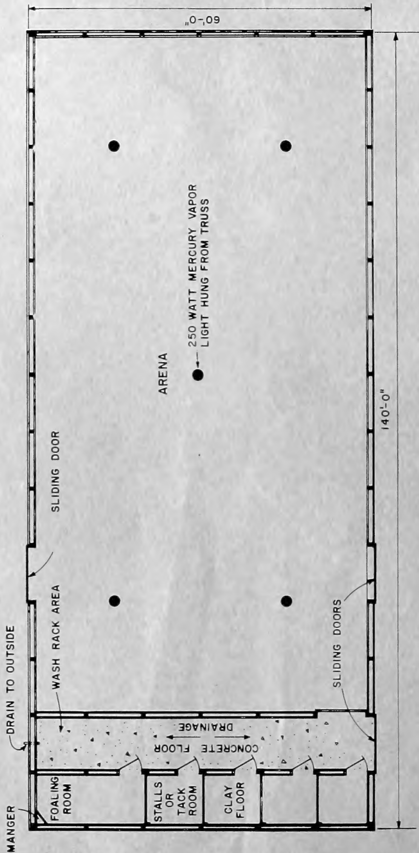
FLOOR PLAN
