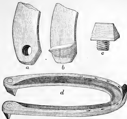
FIG. 8.—WHITE'S PLAN OF ROUGHING SHOES.
