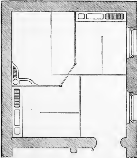
PLAN OF STABLE FOR THREE HORSES.
