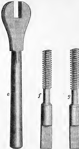
FIG. 2.—SPANNER AND TAPS FOR ROUGHING. e. Spanner. f. g. Taps for tapping. \frac{1}{4} inch size.
