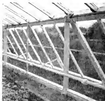
This photo taken in Antoine Schulteis' new house at College Point, L. I., proves that you get same width opening as with the old style equipment.
