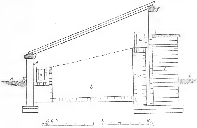
Fig. 336. Section of the pine pit at Oakhill.
