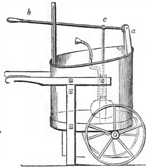
Fig. 83. Read's barrow engine.
