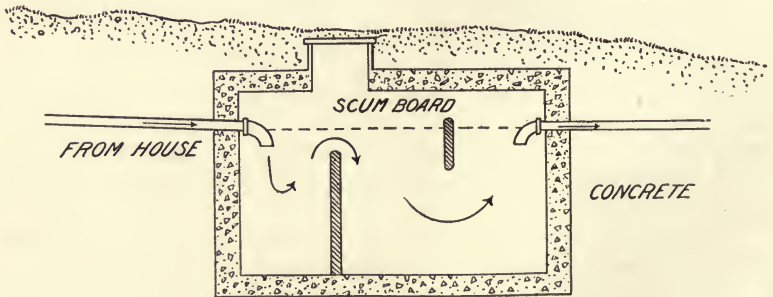
FIG. 24.—Septic tank.
