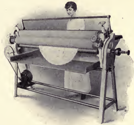
FIG. 83.—Flat-work ironer.
