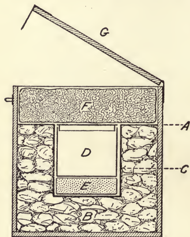
FIG. 58.—Home-made fireless cooker. A , outside container-box or trunk; B , insulating material—paper, sawdust, cinders; C , metal lining of nest—tin, zinc, aluminum; D , cooking kettle—aluminum, agate; E , soap-stone plate, or some heat-containing material; F , pad of excelsior for covering; G , hinged cover for the top of the outside.
