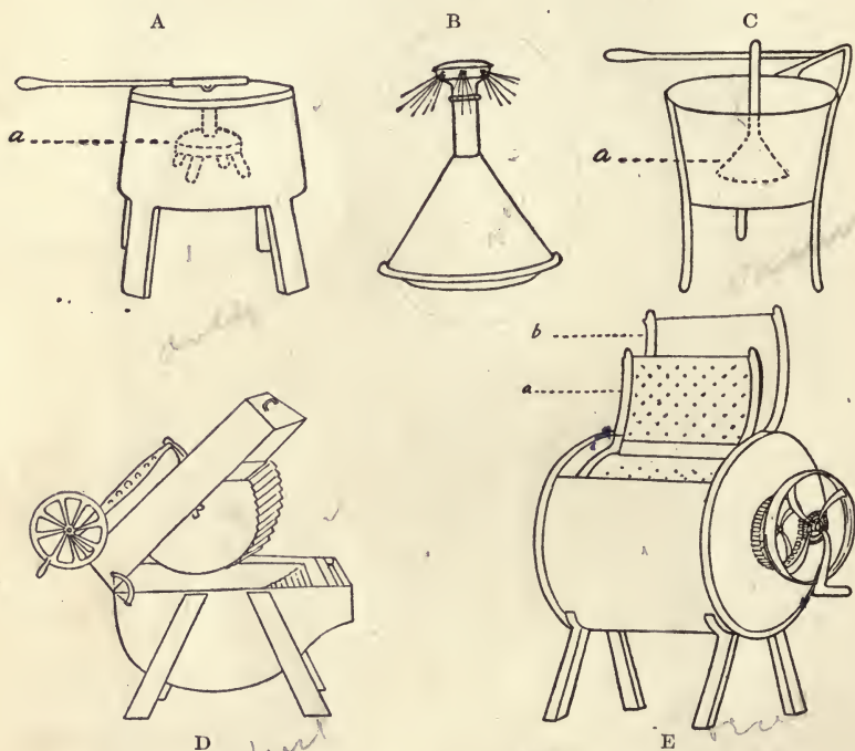
FIG. 73.—Types of washing machines. A , the Dolly type, a , dolly; B , a vacuum boiler washer; C , pressure and suction type, a , funnel; D , washer with corrugated lining; E , a revolving cylinder type; a , inner cylinder perforated; b , outer cylinder—wooden or copper. Courtesy Country Gentleman .
