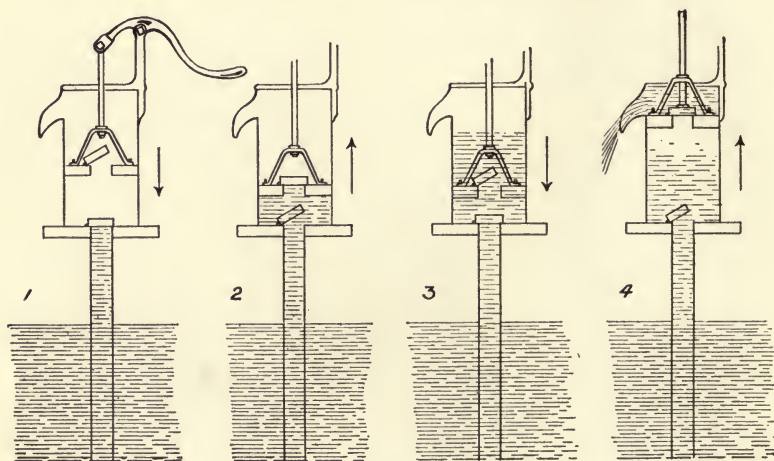
FIG. 12.—Piston pump.
