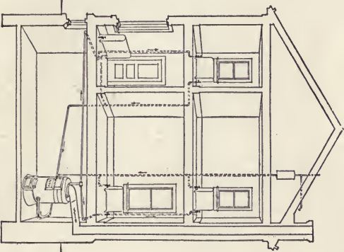
Fig. 47.—A hot-water system depends upon the cold water pushing the hot water to top, because it is lighter and the cold enters at the bottom. To take care of the water expansion, a tank is located near the roof with a vent for an overflow.
