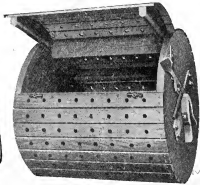
FIG. 75.—Rotary washer. The clothes are put in this inner cage which revolves in the soap and water. The action of the cage reverses, and the load should not be so full that the clothes do not drop on each revolution. The "drop" causes a displacement of the dirt.
