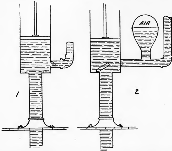
FIG. 13.—Types of force pumps. 1, water goes out on the down stroke; 2, water goes out on both up and down strokes.
