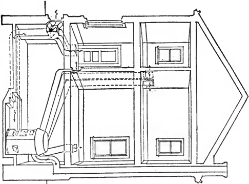
Fig. 46.—A hot air furnace should be located near the coldest part of the house and as centrally as possible. In order to give the leader pipes the maximum upward slope, the cellar should be deep or the furnace put in a pit (If a pit is used, provide for its drainage.)
