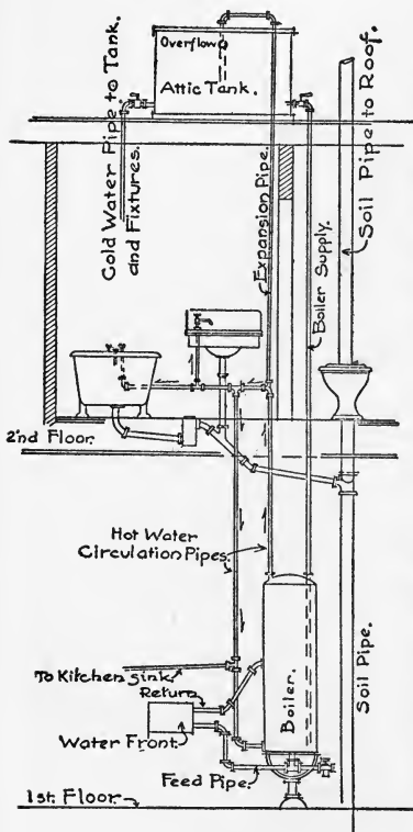
FIG. 50.—Hot-water circulation.
