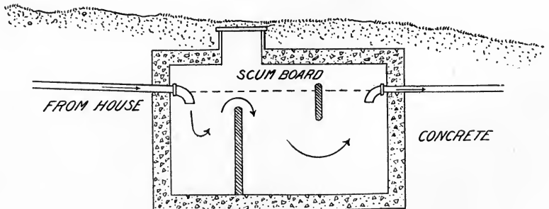
FIG. 24.—Septic tank.
