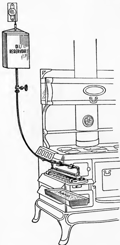
FIG. 43.—A device for burning kerosene in the cook stove.
