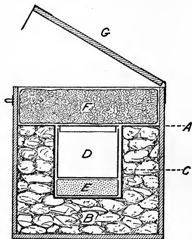
FIG. 58.—Home-made fireless cooker. A, outside container-box or trunk; B, insulating material—paper, sawdust, cinders; C, metal lining of nest—tin, zinc, aluminum; D, cooking kettle—aluminum, agate; E, soapstone plate, or some heat-containing material; F, pad of excelsior for covering; G, hinged cover for the top of the outside.
