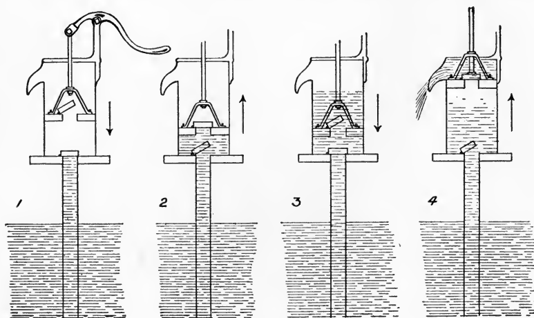
FIG. 12.—Piston pump.
