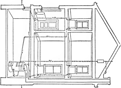
Fig. 47.—A hot-water system depends upon the cold water pushing the hot water to the top, because it is lighter and the cold water at the bottom. To take care of the water expansion, a tank is located near the roof with a vent for an overflow.
