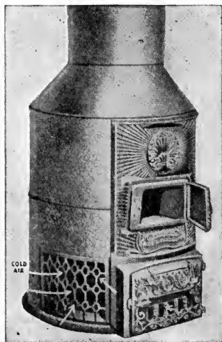
FIG. 48a.—One pipe heater
