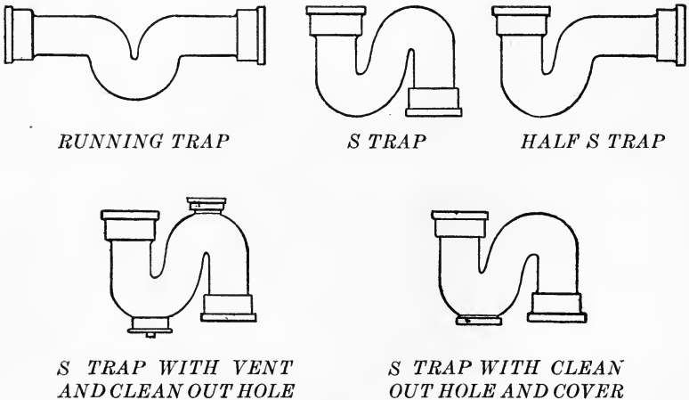
FIG. 21.—Types of traps.
