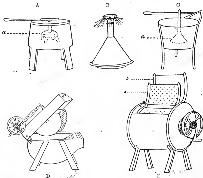
FIG. 73.—Types of washing machines. A, the Dolly type, a, dolly; B, a vacuum boiler washer; C, pressure and suction type, a, funnel; D, washer with corrugated lining; E, a revolving cylinder type; a, inner cylinder perforated; b, outer cylinder—wooden or copper. Courtesy Country Gentleman .
