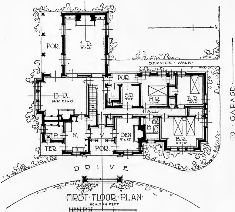
FIG. 6.—Farmhouse. The good feature of this plan is that it is a compact bungalow plan with each unit so distinct that it may be entirely closed off. Planning the kitchen to face the road adds cheer.
