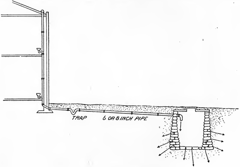
FIG. 23.—Leaching cess-pool.
