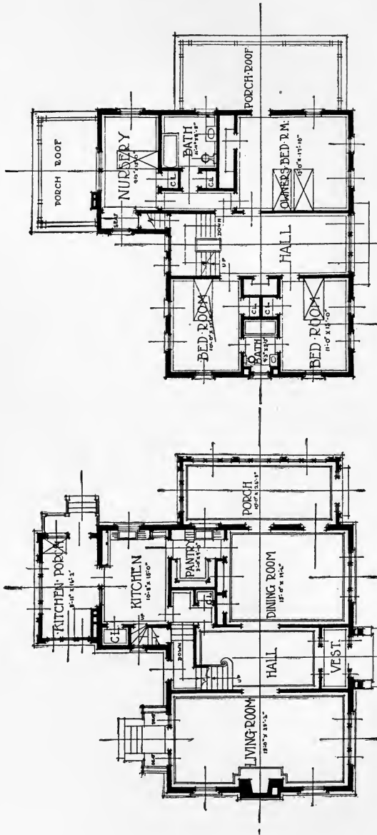
FIRST FLOOR PLAN SECOND FLOOR PLAN Fig. 7.—Colonial house. Good plan for efficiency and comfort.
