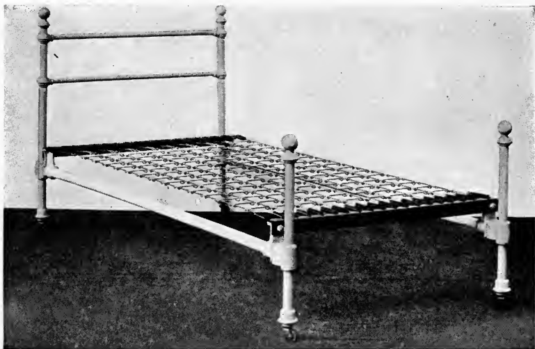
FIG. 119.—A national spring which may be repaired by replacing the springs at each end or by putting in new links.
