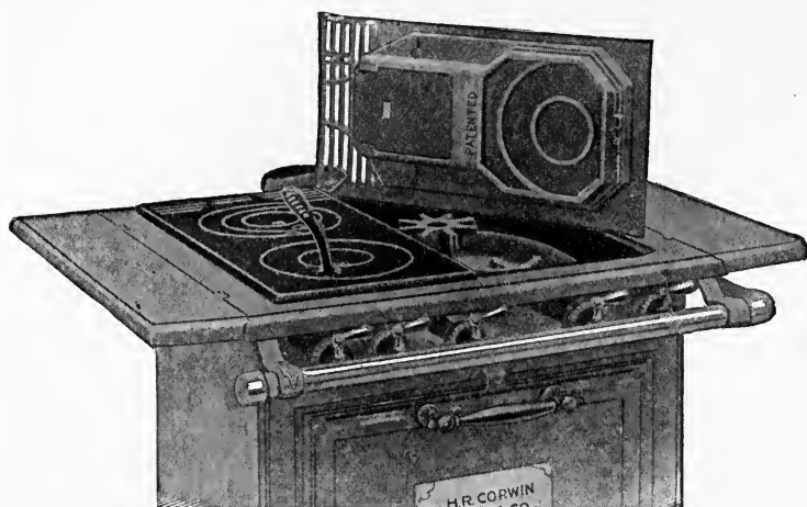
FIG. 55.—Cast-iron top for a gas stove. This is a good means of saving gas. The heat of the flame under the front burner is sufficient for slow cooking on the back burner. Such a top makes the gas stove top like the coal stove.
