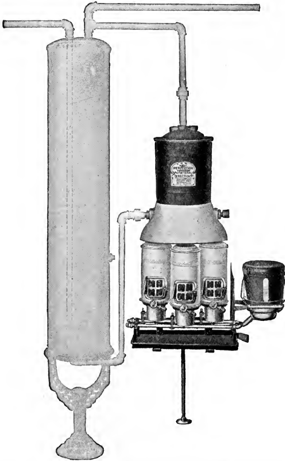
FIG. 53.—Blue flame hot-water heater. Such a heater gives great service in houses where there is no coal range and where a kerosene cookstove is used entirely.
