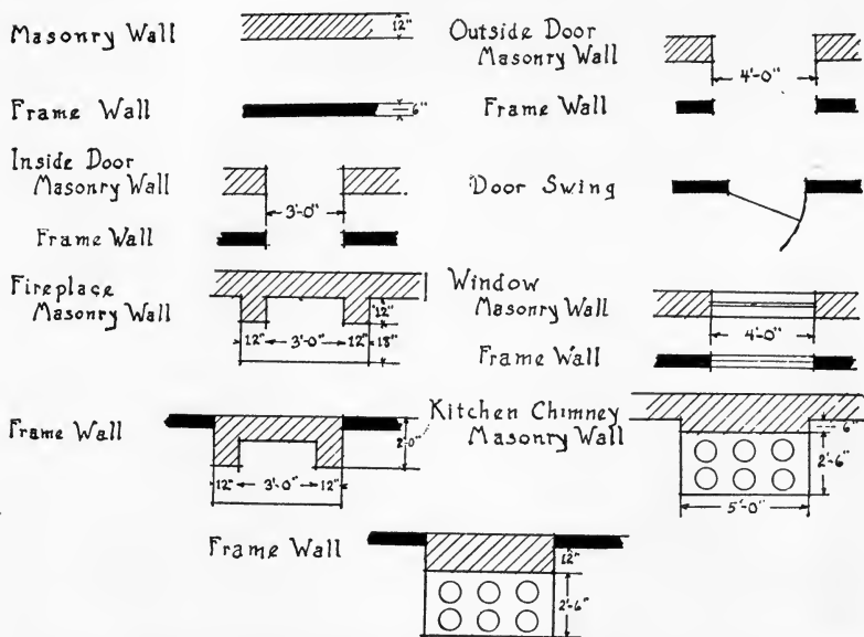
FIG. 1.—Architect's method of indicating houseplans. Easily drawn on special paper which is blocked off in quarter inch squares. Allow 1/4 inch for a foot.
