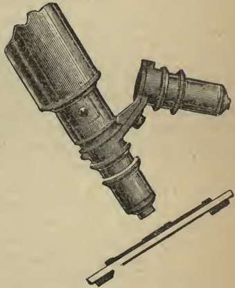
Fig. 42.—BENT NOSE-PIECE.
