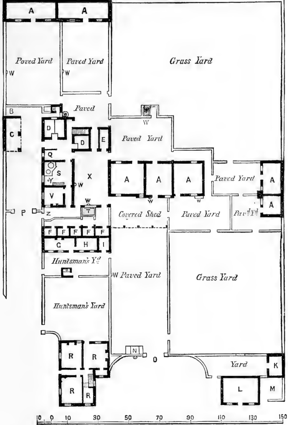
PLAN OF KENNELS, BADMINTON.
