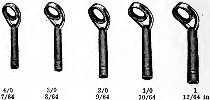
"Dowagiac" pattern agate casting tip-guide
