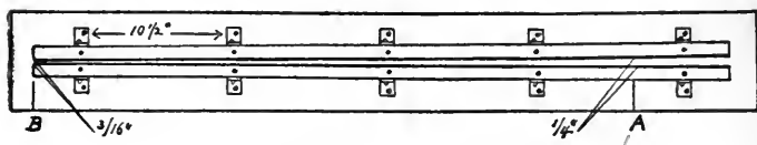
Fig. 2 — Top view of steel planing-mold
