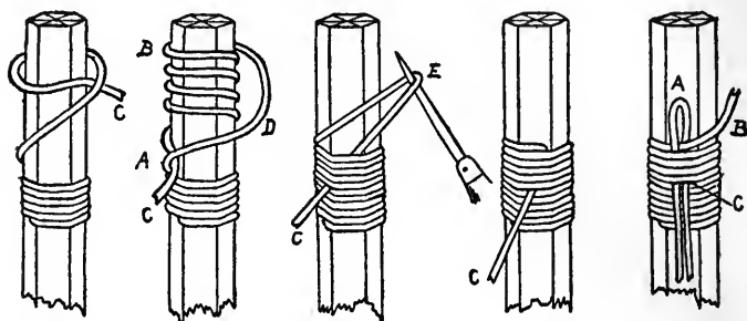
Fig. 1 Fig. 2 Fig. 3 Fig. 4 Fig. 5 Silk winding: (1) Starting the loose coils; (2) Free end of silk run under; (3) Loose coils wound tightly over terminal end — awl-point holds loop; (4) The loop drawn in; (5) Separate-loop method
